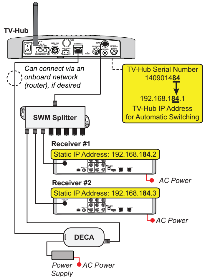
Figure 57: IP Addressing for Automatic Switching (Example)
