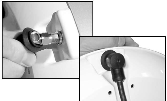
Figure 11: Protecting the Connector with the Rubber Boot
