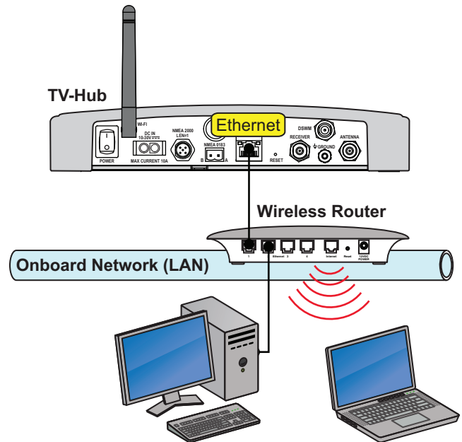
Figure 36: TV-Hub Network Connections
