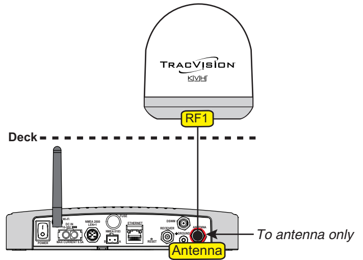
Figure 17: TV-Hub Antenna Connection
