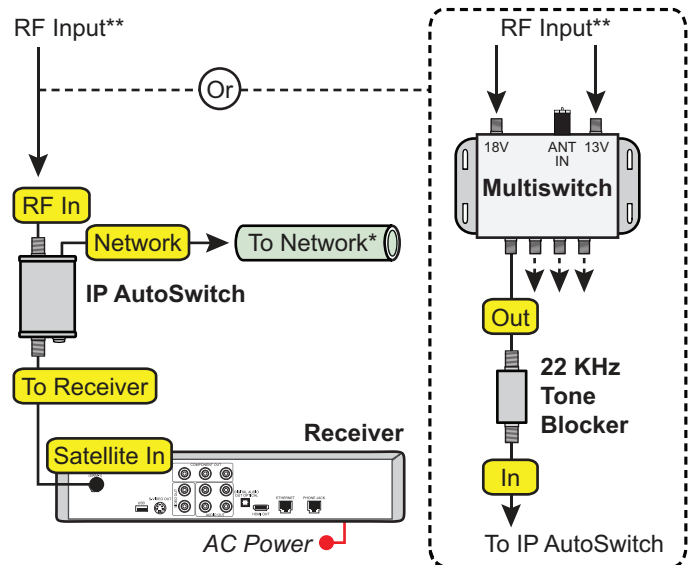
Figure 52: IP AutoSwitch Connections
