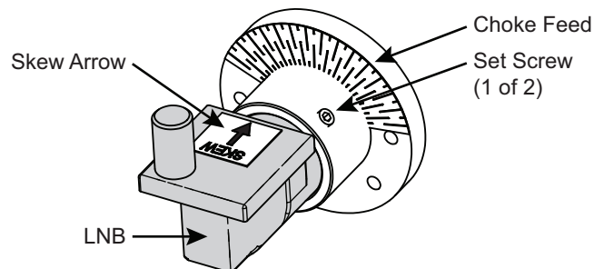
Figure 46: LNB Skew Angle Adjustment
