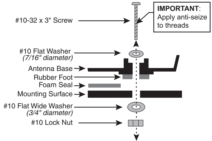
Figure 14: Mounting Hardware
