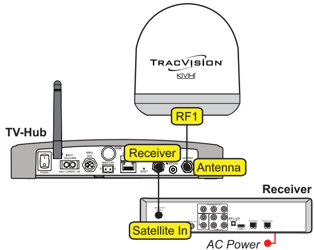
Figure 24: Wiring 1 DISH/Bell Receiver
