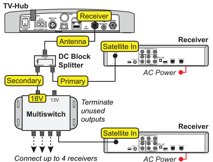
Figure 26: Wiring 3+ DISH/Bell Receivers
