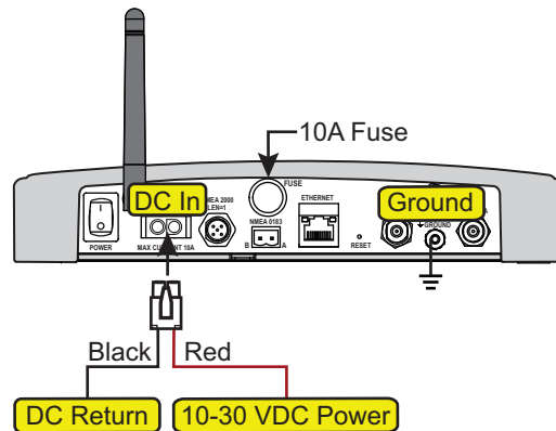
Figure 31: TracVision System Power
