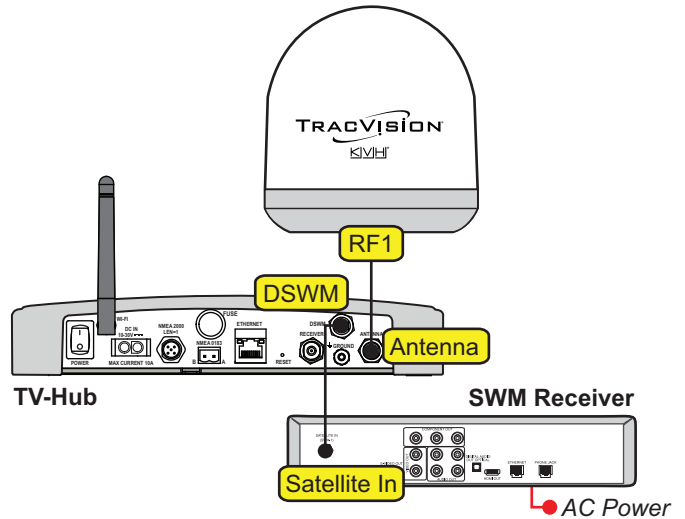
Figure 22: Wiring Up to 8 SWM Devices
