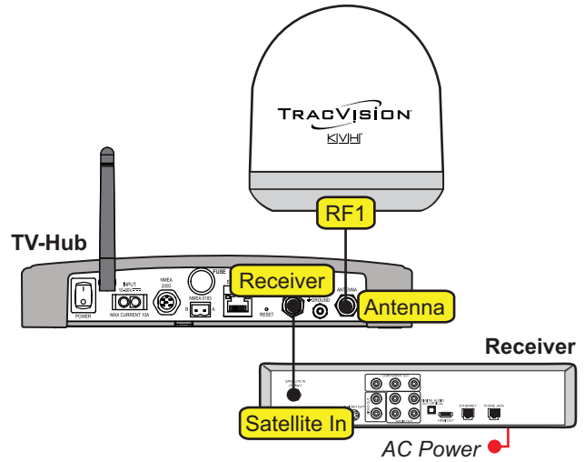
Figure 20: Wiring a Linear Receiver
