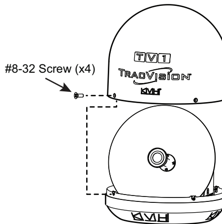
Figure 12: Removing the Radome
