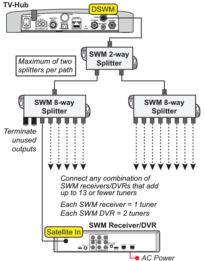
Figure 23: Wiring Up to 13 DIRECTV SWM Devices
