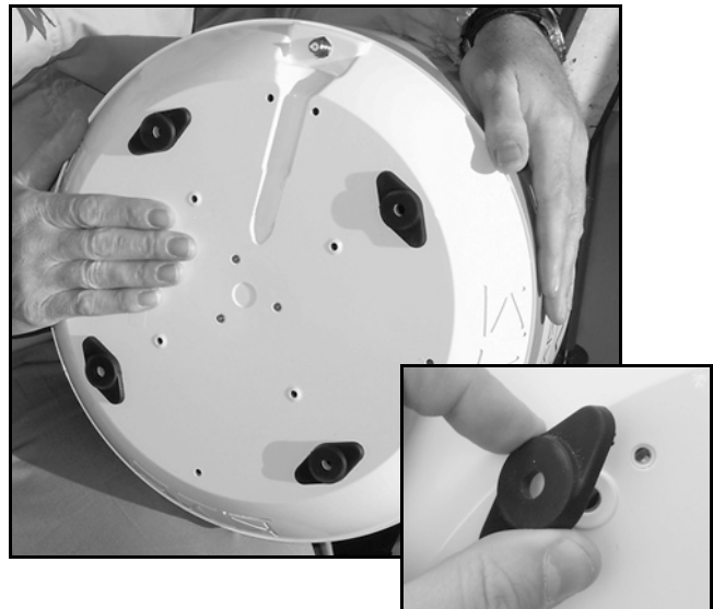
Figure 9: Attaching the Rubber Feet
