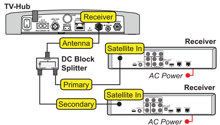
Figure 25: Wiring 2 DISH/Bell Receivers
