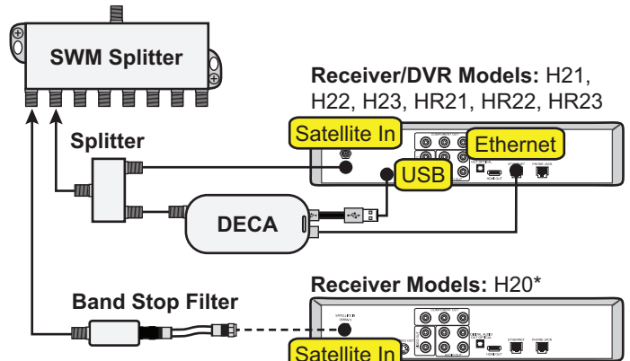
Figure 56: Additional Equipment for Older Receivers
