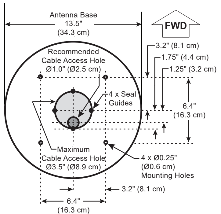
Figure 7: Antenna Mounting Holes Layout
