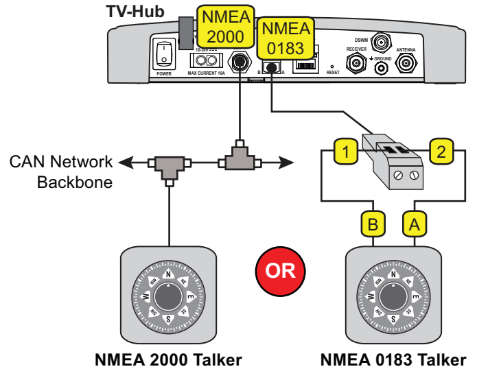
Figure 27: TV-Hub NMEA Connections
