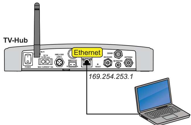
Figure 35: Wired Ethernet Connection
