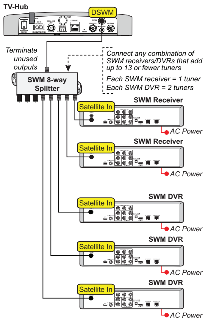
Figure 22: Wiring Up to 8 SWM Devices
