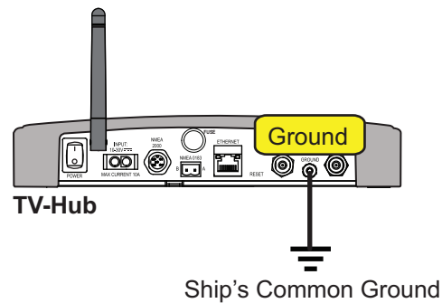
Figure 30: TV-Hub Grounding Connections
