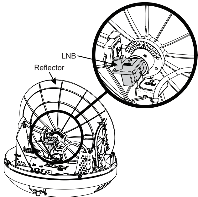
Figure 46: LNB Skew Angle Adjustment
