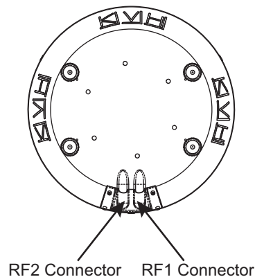
Figure 13: Connectors on Bottom of Dual Linear Antenna
