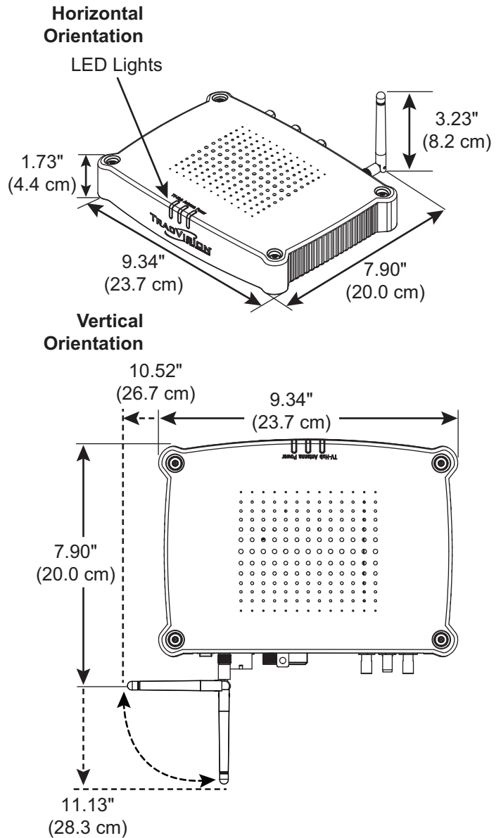
Figure 6: TV-Hub Dimensions
