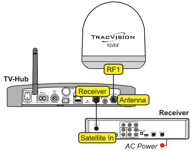
Figure 23: Wiring 1 Linear Receiver
