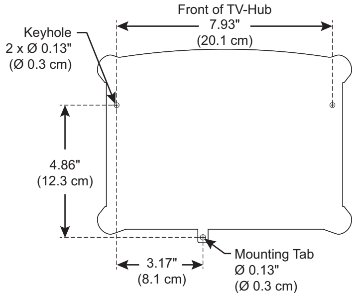
Figure 18: TV-Hub Mounting Template
