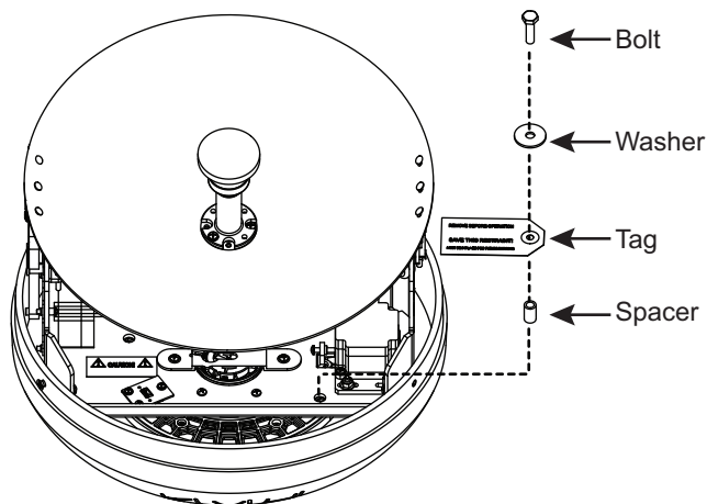
Figure 15: Shipping Restraint Hardware
