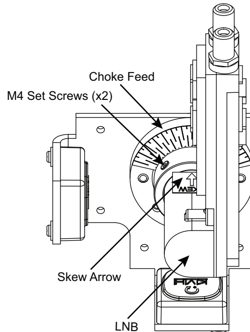
Figure 49: LNB Set Screws and Skew Angle Adjustment
