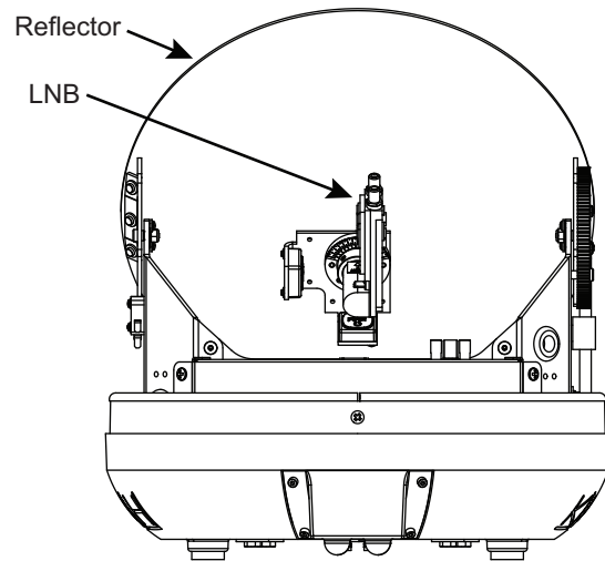
Figure 48: Location of LNB on Back of Antenna Reflector
