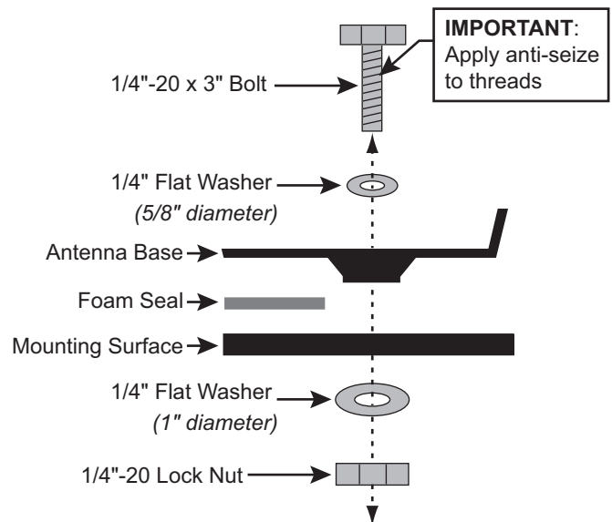
Figure 17: Mounting the Antenna (Side View)
