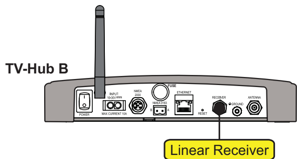
Figure 22: TV-Hub B Receiver Connections
