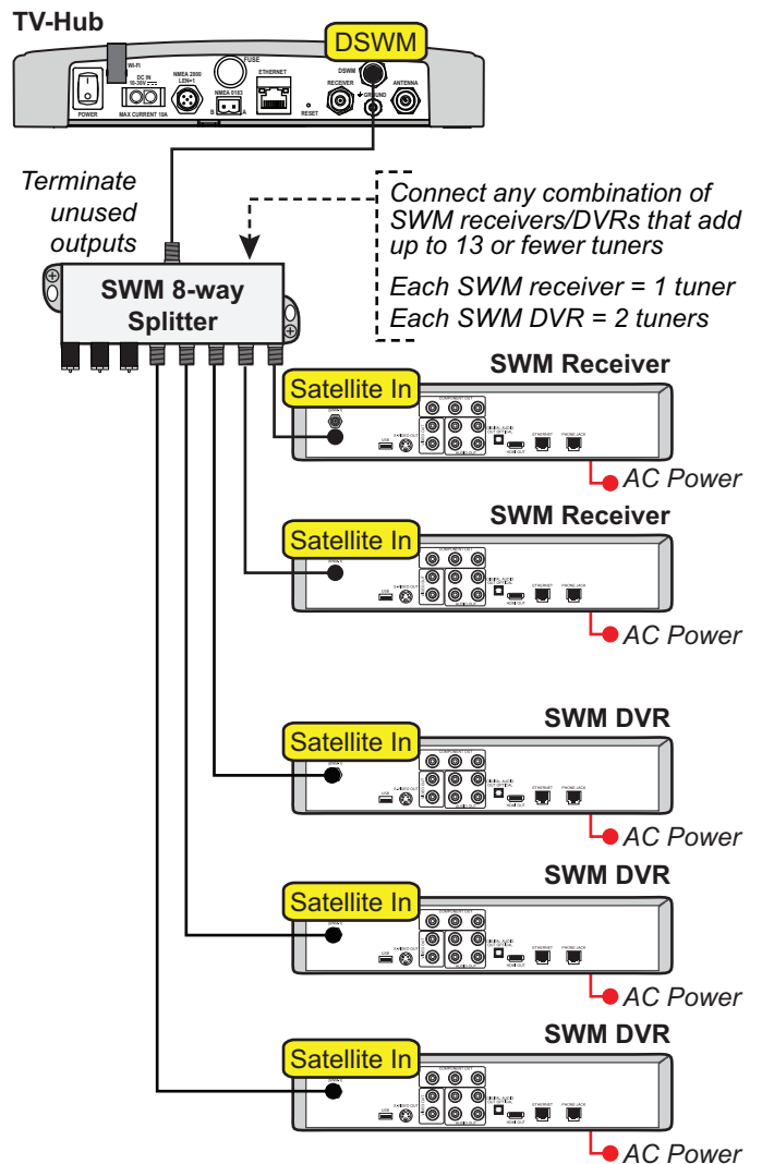
Figure 26: Wiring Up to 8 SWM Devices
