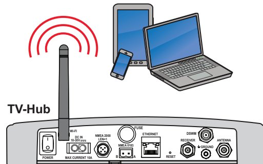
Figure 38: Wi-Fi Connection
