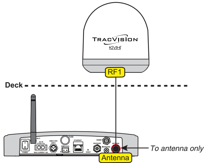
Figure 20: TV-Hub Antenna Connection
