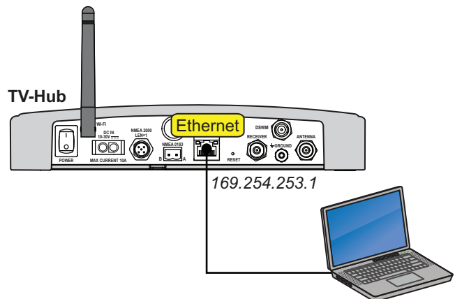
Figure 39: Wired Ethernet Connection
