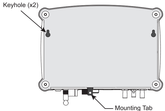
Figure 19: TV-Hub Keyholes and Mounting Tab
