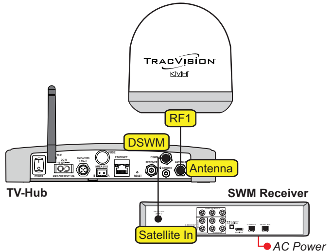
Figure 26: Wiring Up to 8 SWM Devices
