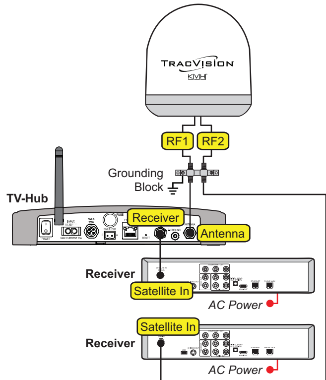
Figure 24: Wiring 2 Linear Receivers (Dual Linear System Only)
