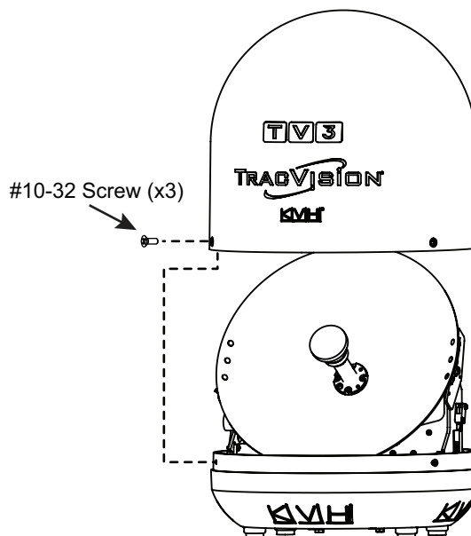
Figure 14: Removing the Radome
