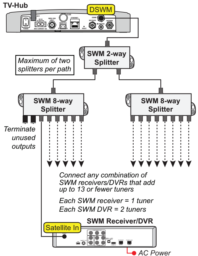
Figure 27: Wiring Up to 13 DIRECTV SWM Devices
