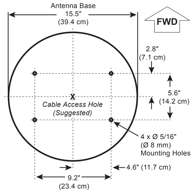
Figure 7: Antenna Mounting Holes Layout
