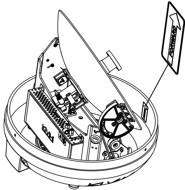
Figure 16: Forward Arrow in Antenna Baseplate
