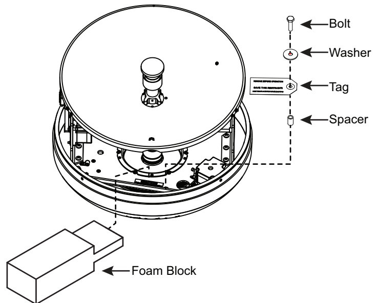
Figure 12: Shipping Restraints
