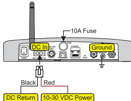
Figure 35: TracVision System Power
