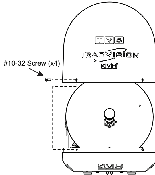
Figure 11: Removing the Radome
