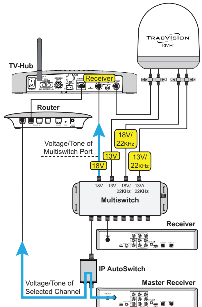
Figure 60: Linear Receivers with Multiswitch and IP AutoSwitch
