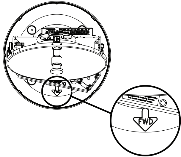
Figure 13: Overhead View of Forward Arrow in Antenna Baseplate
