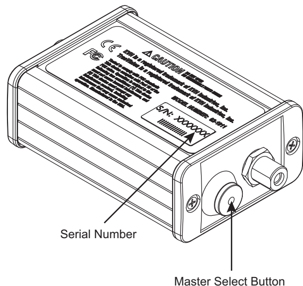
Figure 55: Serial Number and Master Select Button
