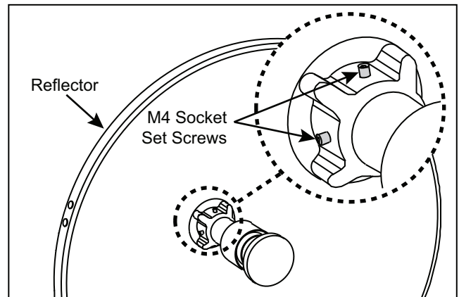
Figure 50: LNB Skew Angle Adjustment
