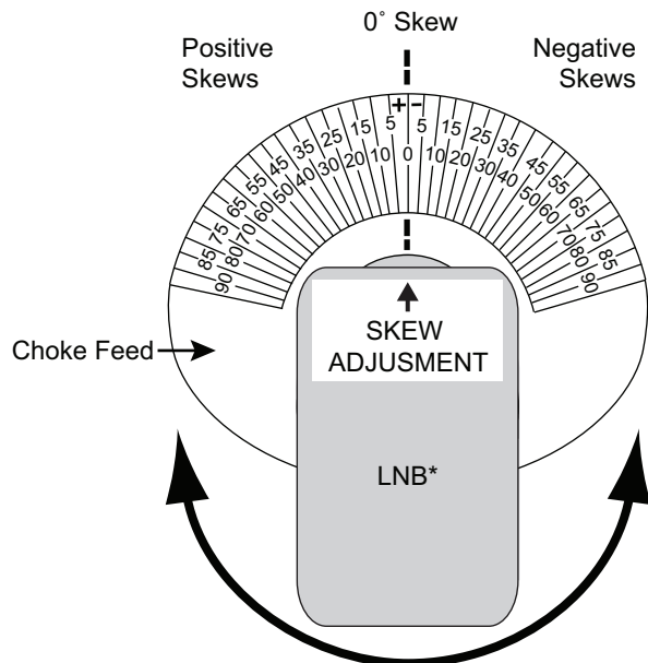
Figure 50: LNB Skew Angle Adjustment
