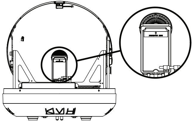
Figure 49: Set Screws Securing the LNB to the Reflector
