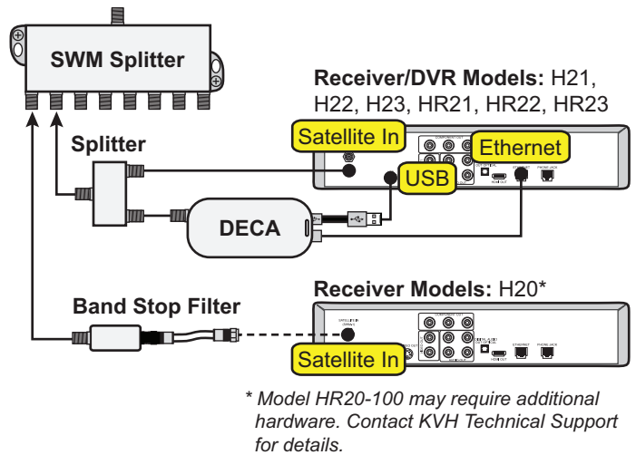
Figure 62: Additional Equipment for Older Receivers
