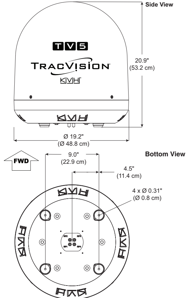
Figure 5: Antenna Dimensions
