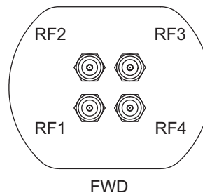
Figure 10: Connectors on Bottom of Antenna
