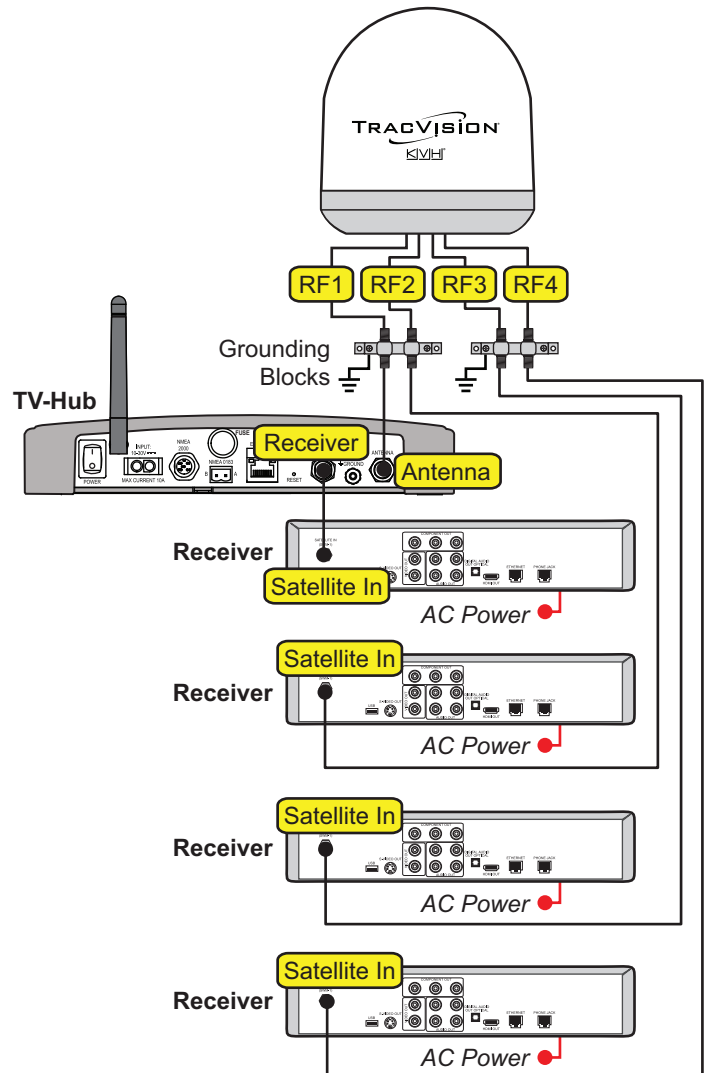
Figure 21: Wiring 2 to 4 Linear Receivers
