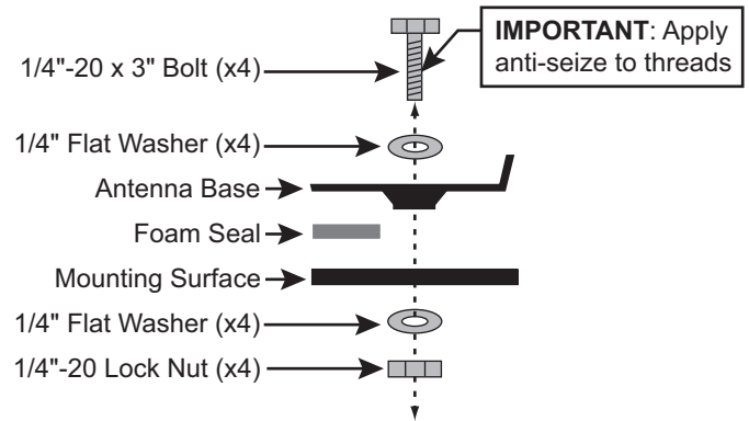
Figure 14: Mounting the Antenna (Side View)
