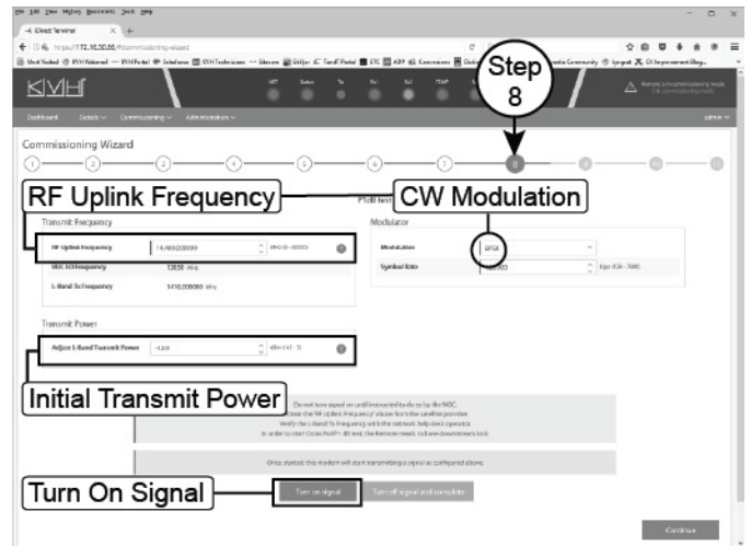
Figure 85: Commissioning – Step 8: CW Modulation continued
