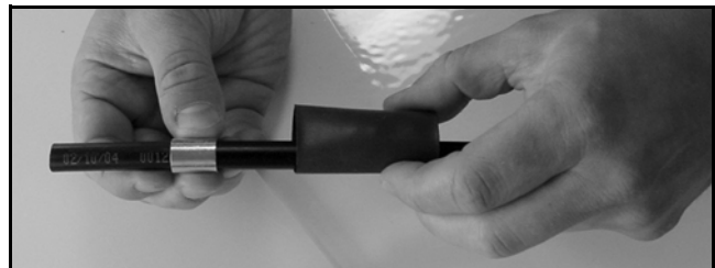
Figure 92: Placing the Heat Shrink Sleeve and Ferrule
