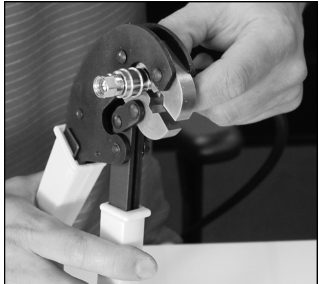
Figure 102: Crimping the Ferrule onto the Cable
