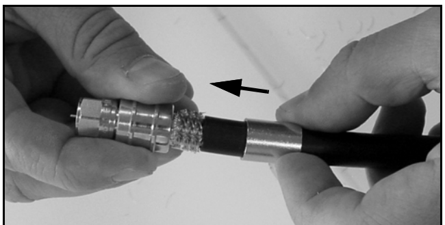
Figure 101: Sliding the Ferrule Over the Braid
