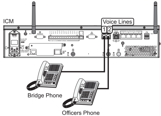
Figure 73: Connecting Vessel Phones (Example)
