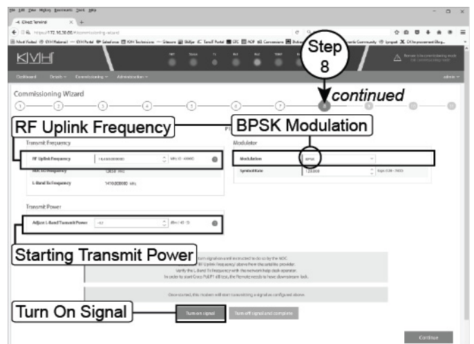
Figure 86: Commissioning – Step 8: BPSK Modulation
