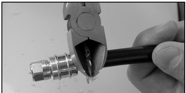
Figure 100: Trimming the Braid
