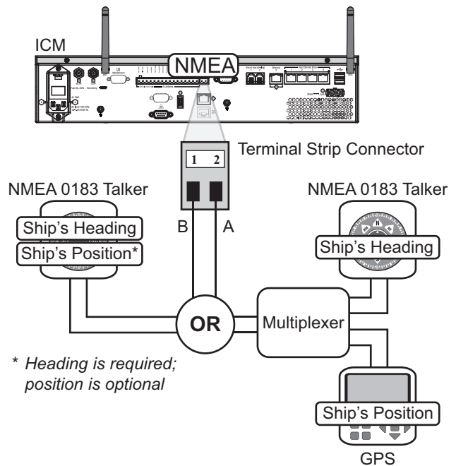
Figure 37: NMEA Wiring
