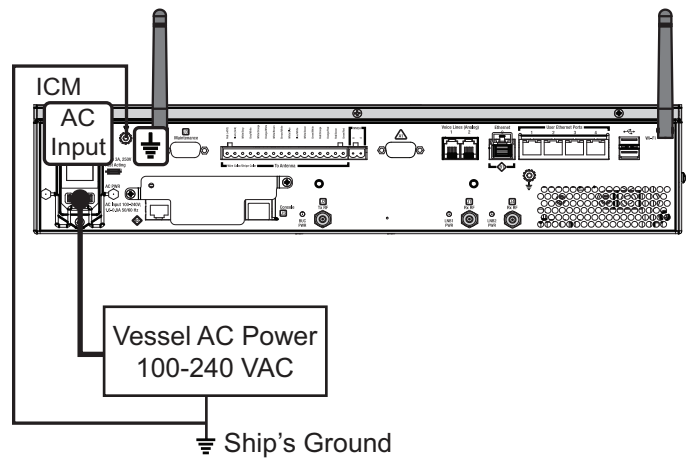
Figure 41: Power Wiring
