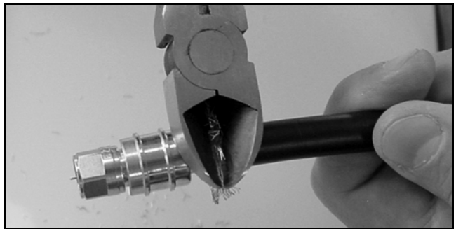
Figure 99: Trimming the Braid
