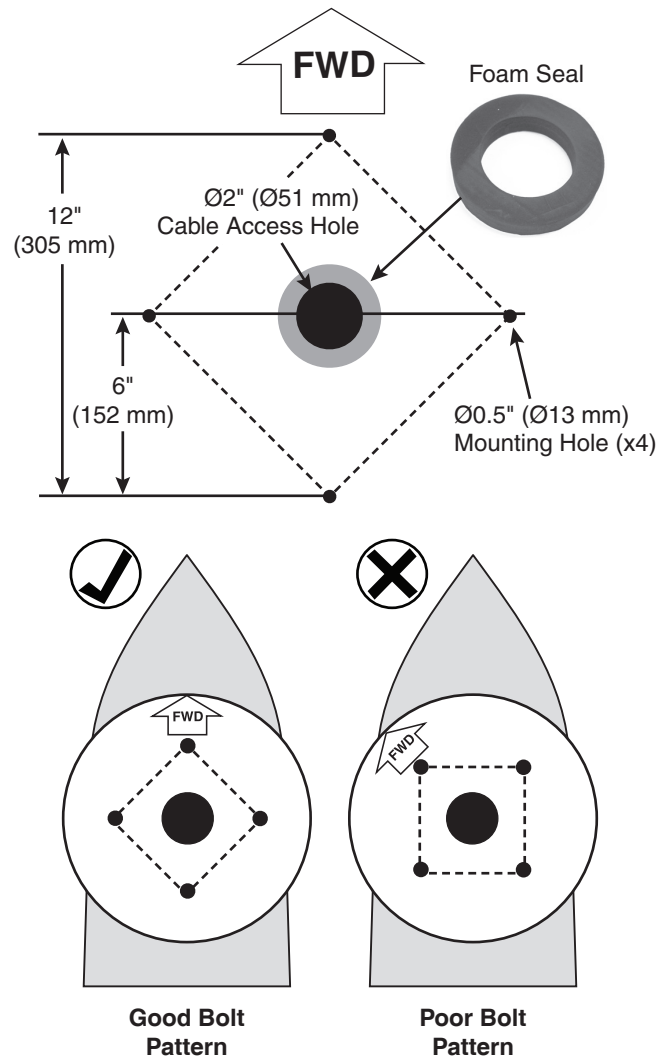
Figure 11: Antenna Mounting Holes Layout
