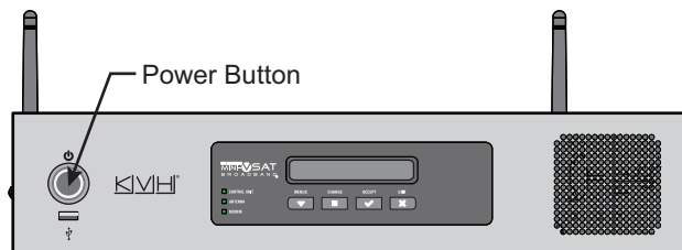
Figure 42: Power Button
