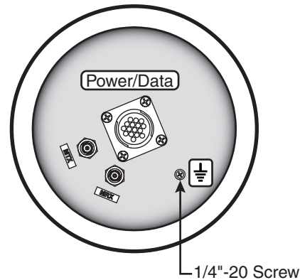
Figure 21: Antenna Power/Data Cable Connections
