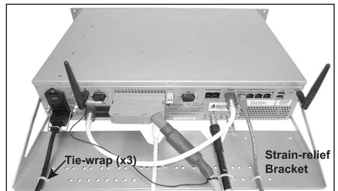
Figure 41: Strain-Relief Bracket
