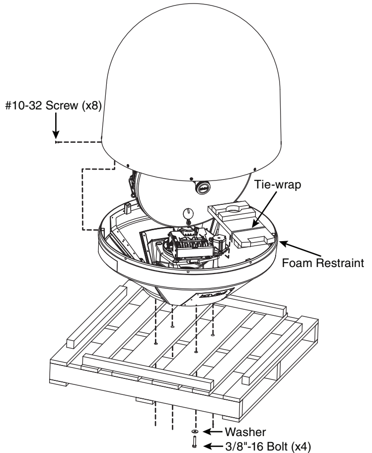
Figure 12: Location of Radome Screws and Restraint Bolts
