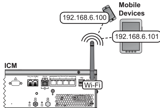
Figure 69: Wireless DHCP (Example)
