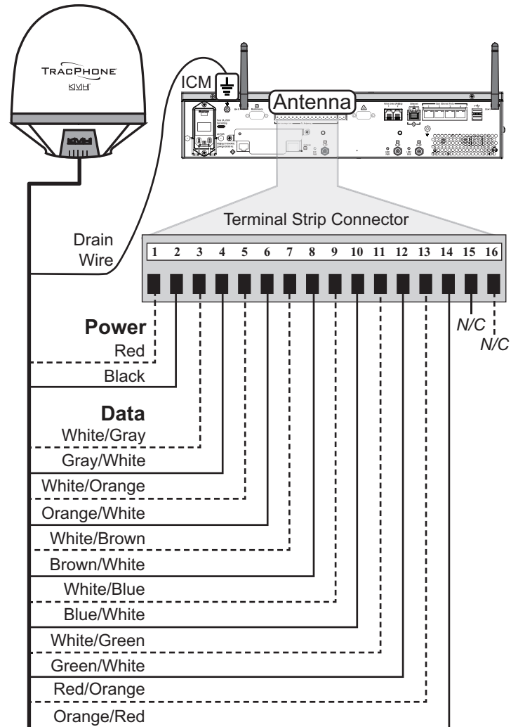
Figure 33: Antenna Power/Data Wiring
