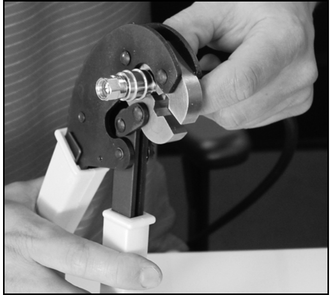
Figure 101: Crimping the Ferrule onto the Cable
