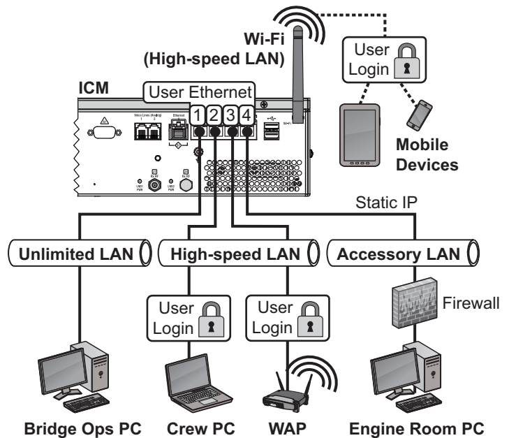
Figure 66: Static IP HTS Configuration Wiring Example
