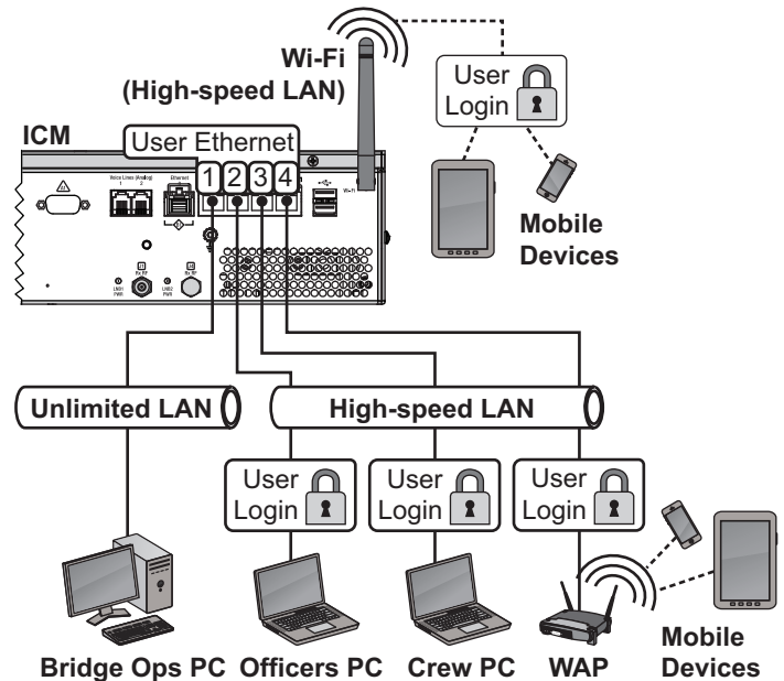
Figure 64: Standard HTS Configuration Wiring Example
