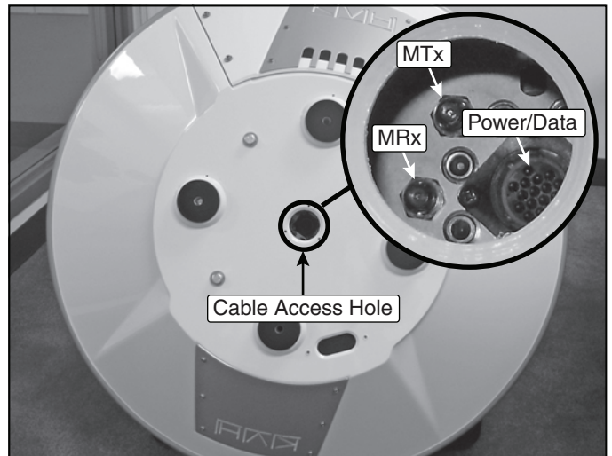
Figure 19: Connectors on Bottom of Antenna
