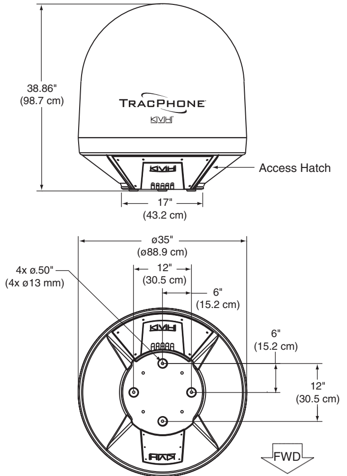
Figure 2: Antenna Dimensions
