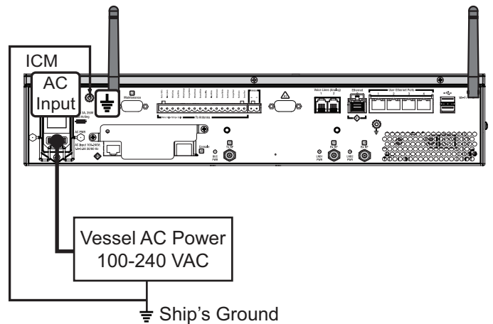
Figure 40: Power Wiring
