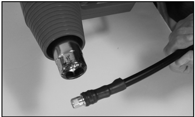
Figure 102: Applying the Heat Shrink Sleeve
