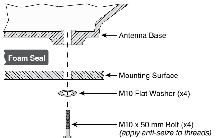
Figure 24: Mounting the Antenna (Side View)
