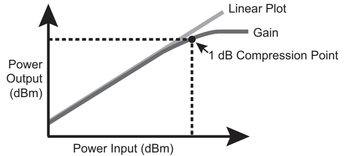
Figure 54: BUC's 1 dB Compression Point Determination
