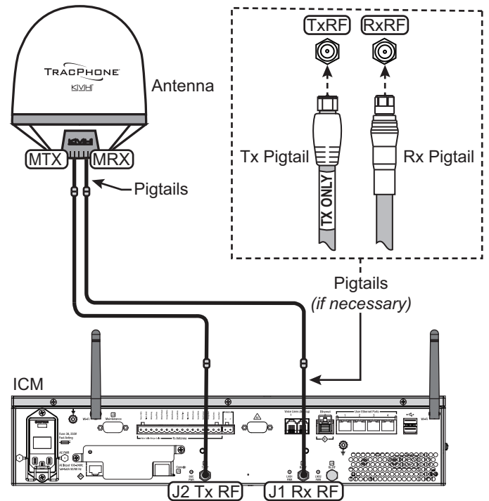
Figure 37: Antenna RF Transmit and Receive Wiring
