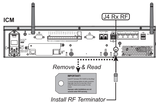
Figure 38: RF Terminator and Instructions Tag
