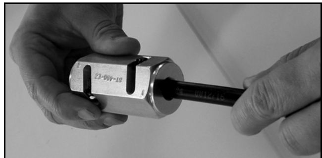
Figure 92: Stripping the End to Expose the Center Conductor
