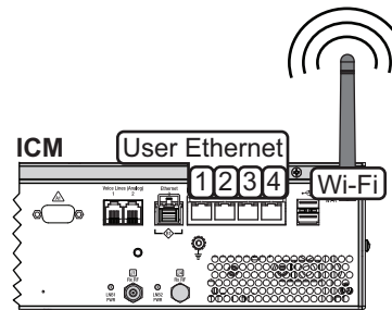
Figure 60: ICM Ethernet Ports and Wireless Access Point
