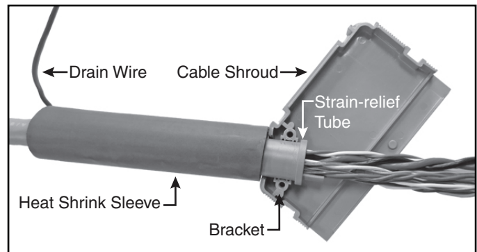
Figure 31: Positioning the Heat Shrink Sleeve
