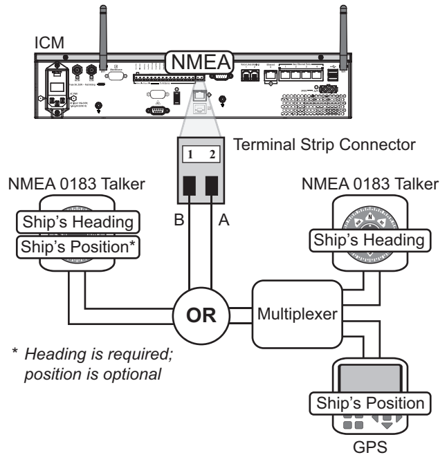
Figure 36: NMEA Wiring
