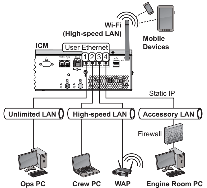
Figure 68: Open Access HTS Configuration Wiring Example
