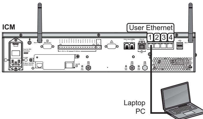
Figure 44: Connecting Your Laptop to the ICM
