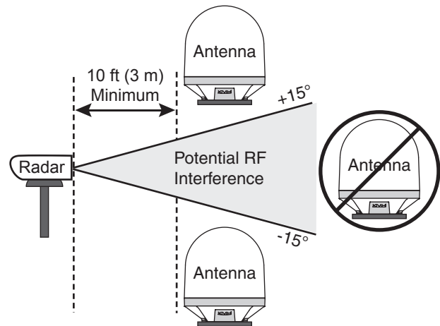
Figure 4: Avoiding RF Interference
