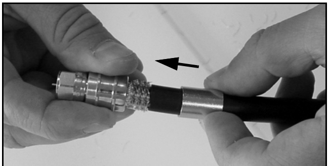
Figure 100: Sliding the Ferrule Over the Braid
