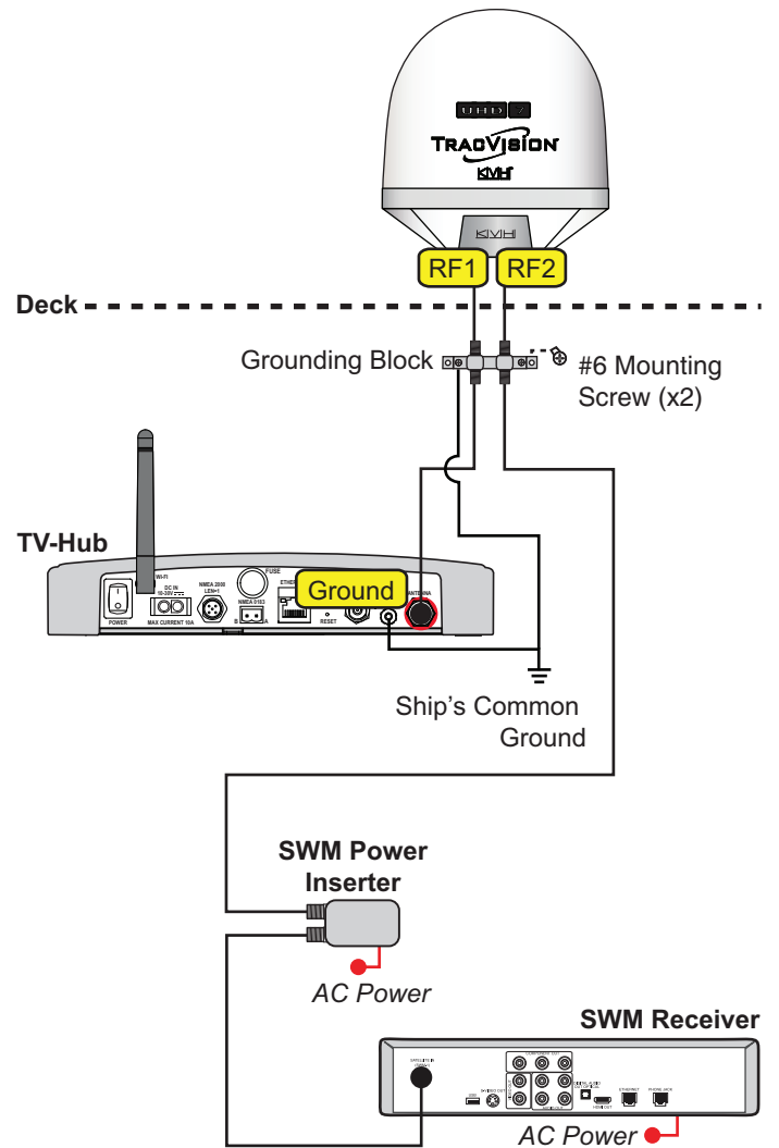
Figure 35: Grounding Block Example
