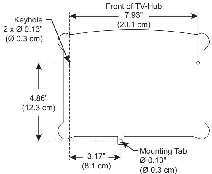
Figure 21: TV-Hub Mounting Template
