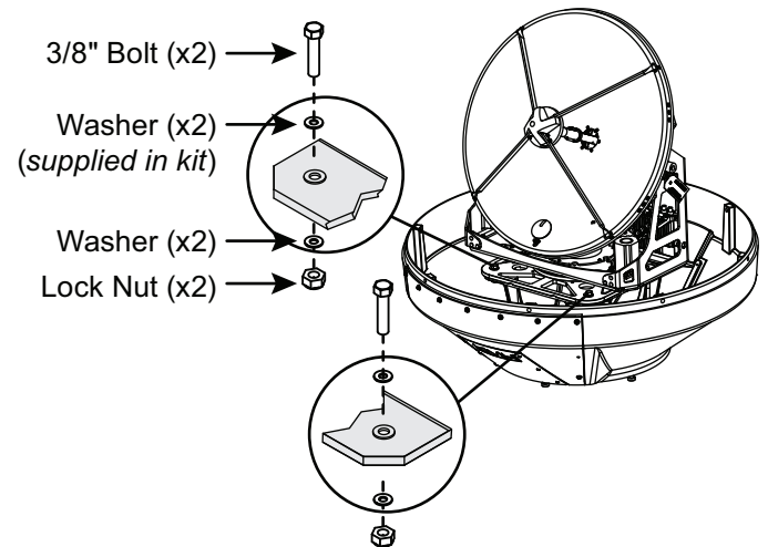
Figure 14: Mounting Bolt Reinstallation
