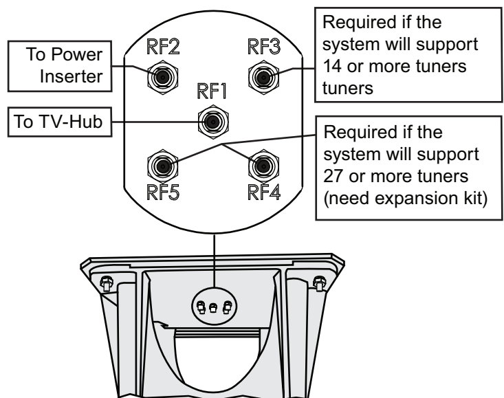
Figure 18: Connectors on Bottom of Antenna
