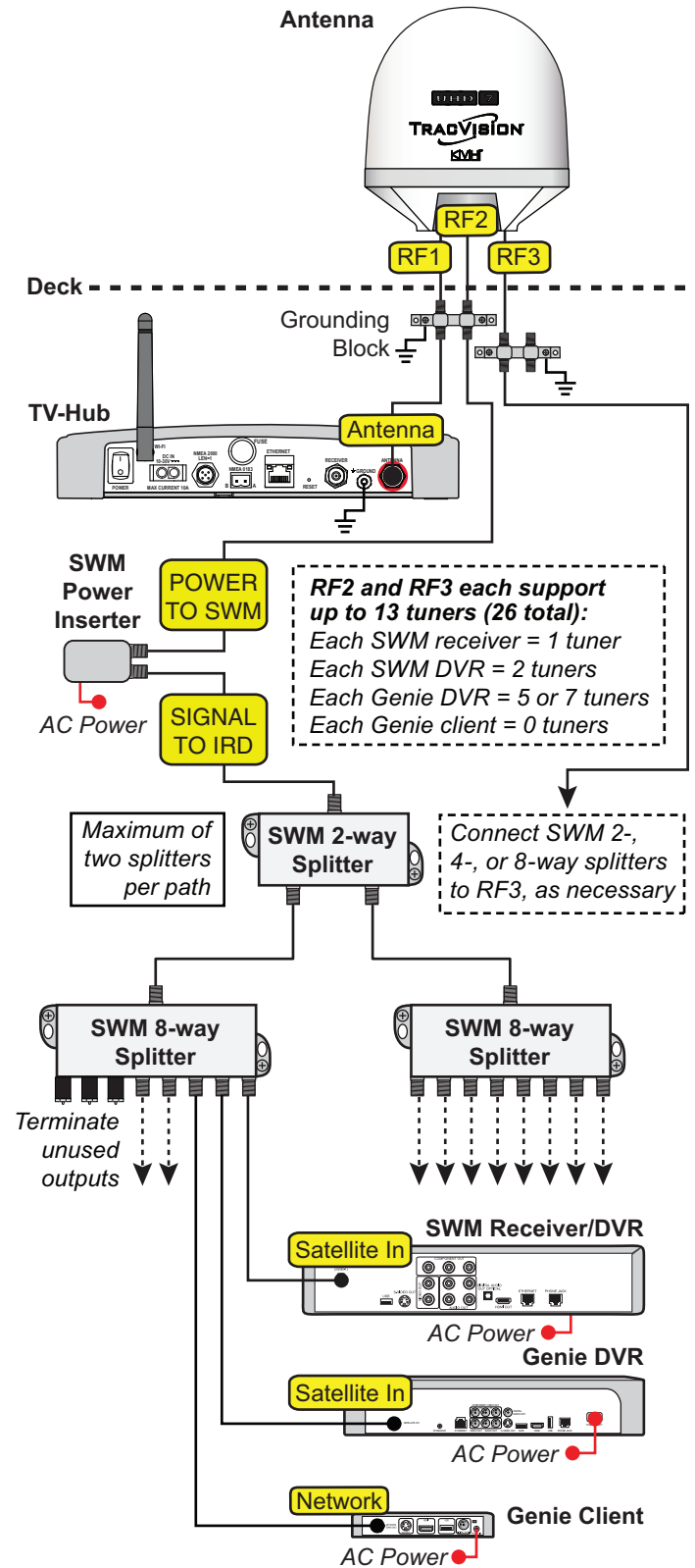
Figure 28: Wiring Up to 26 DIRECTV Receivers
