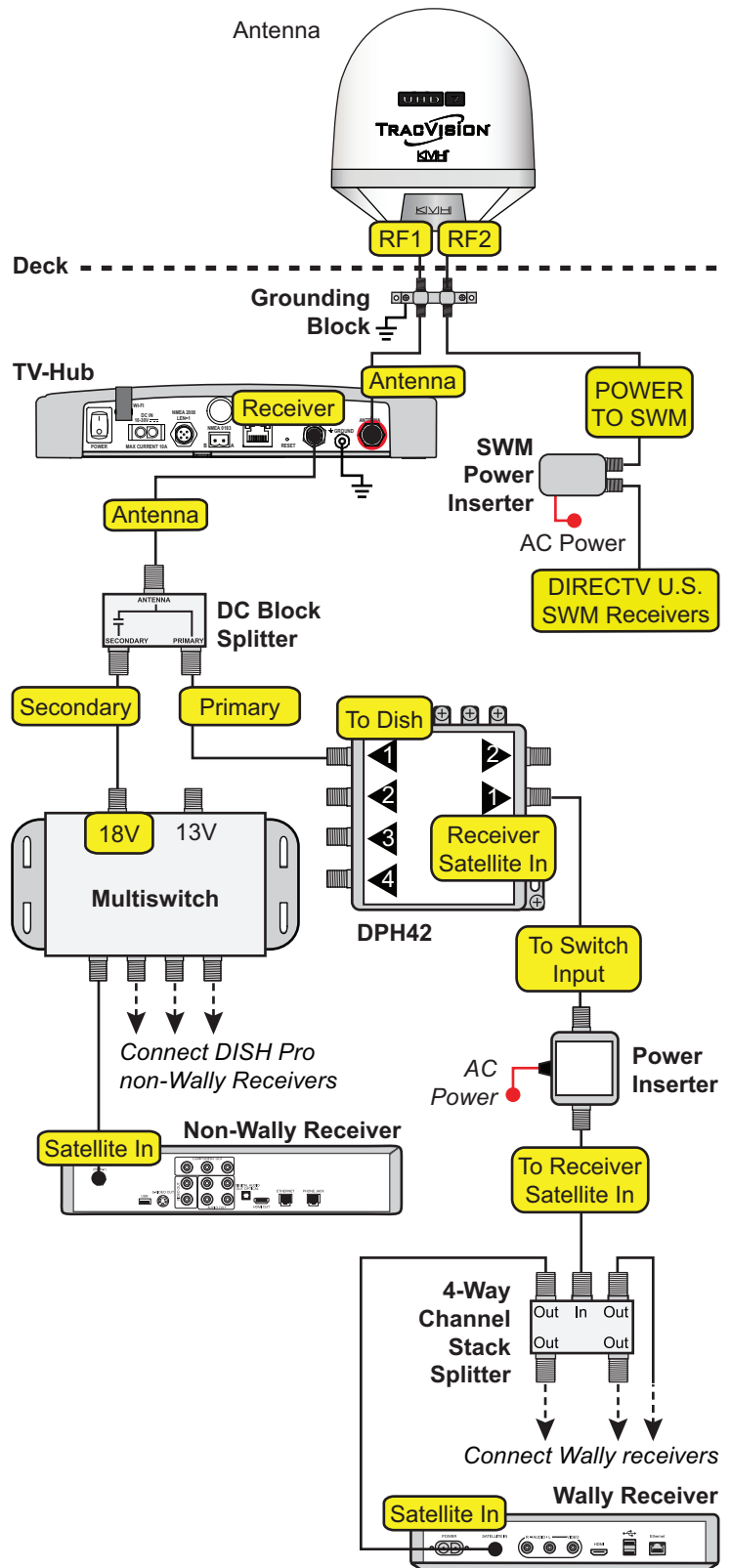
Figure 55: Wiring a Mix of Wally/Non-Wally Receivers
