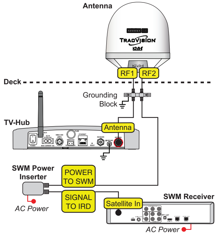
Figure 25: Wiring 1 DIRECTV Receiver
