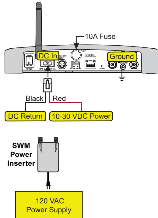
Figure 36: TracVision System Power
