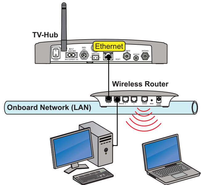
Figure 41: TV-Hub Network Connections
