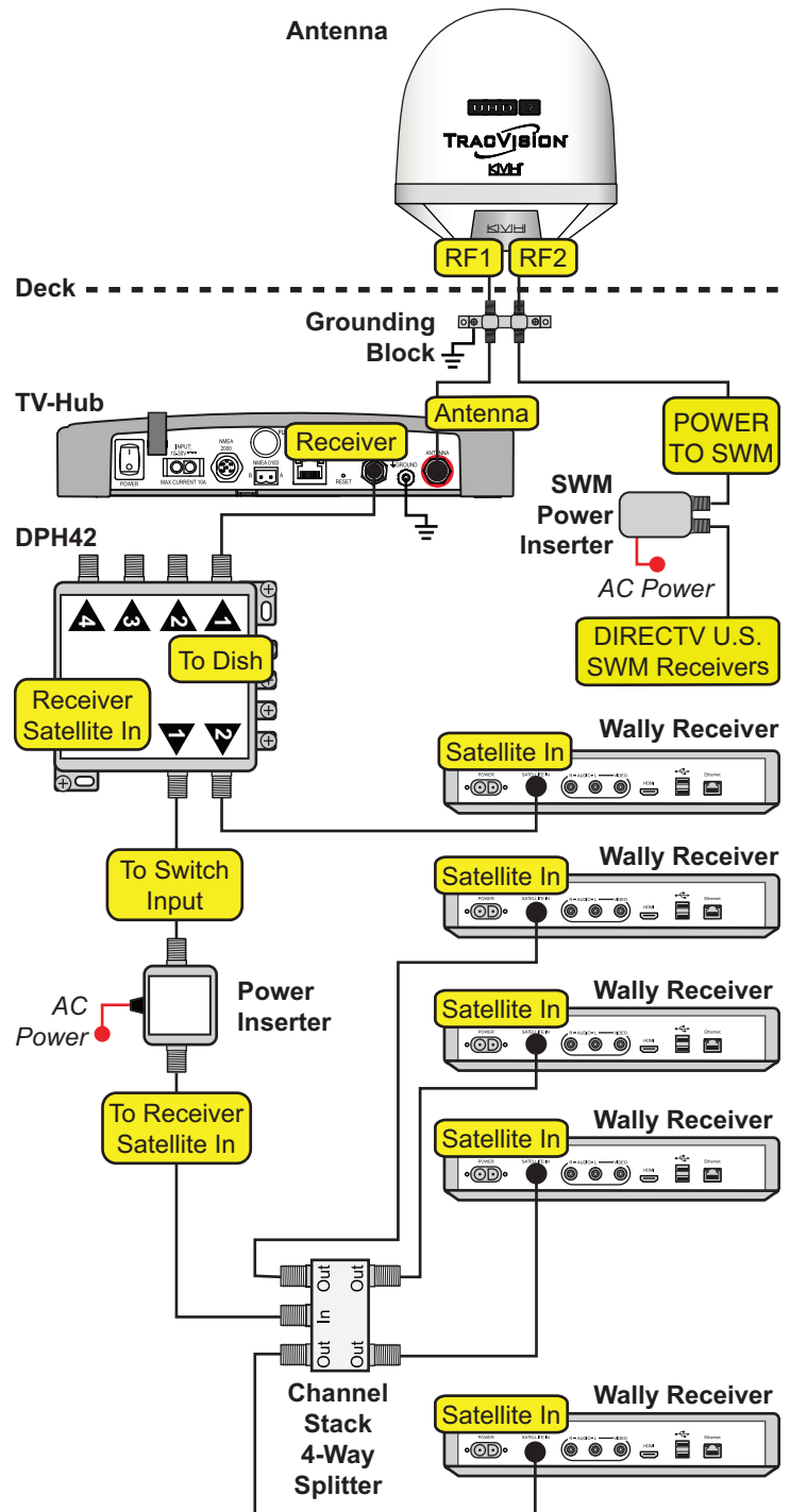
Figure 52: Wiring Up to 5 Wally Receivers
