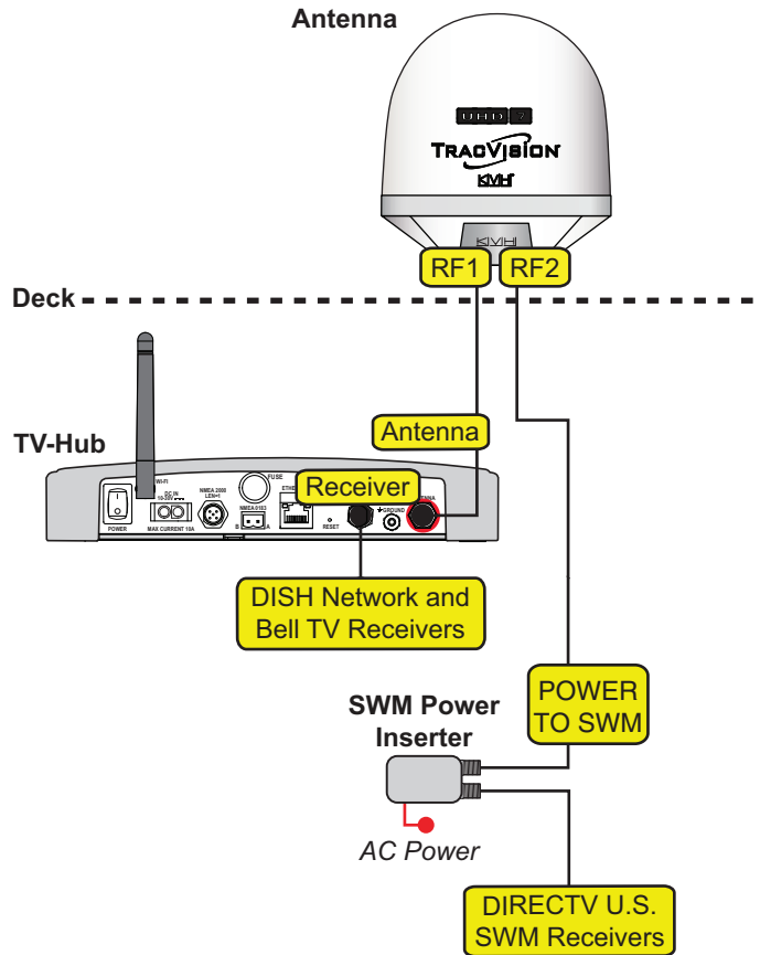
Figure 24: Receiver/DVR Wiring
