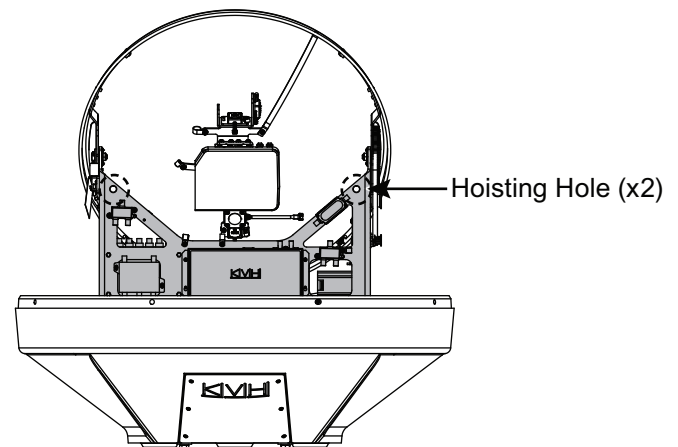
Figure 12: Antenna Hoisting Holes
