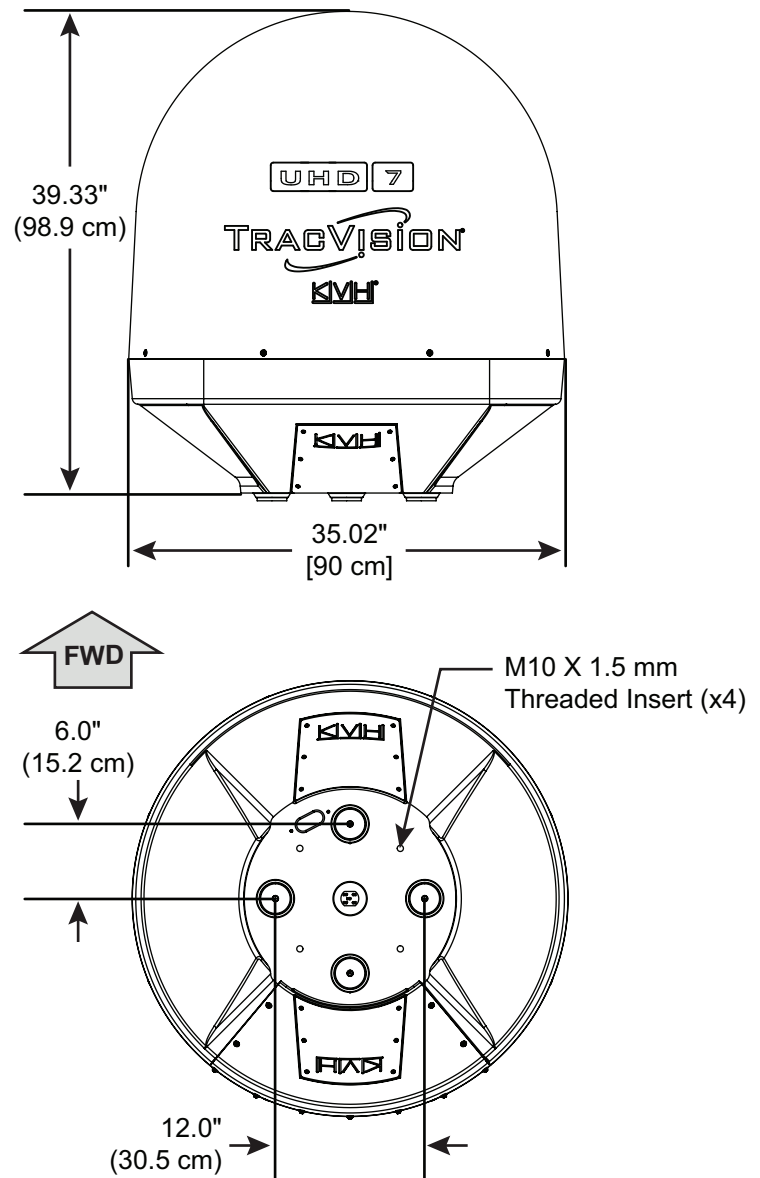
Figure 5: Antenna Dimensions
