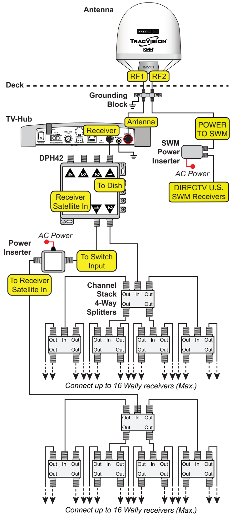
Figure 54: Wiring Up to 32 Wally Receivers
