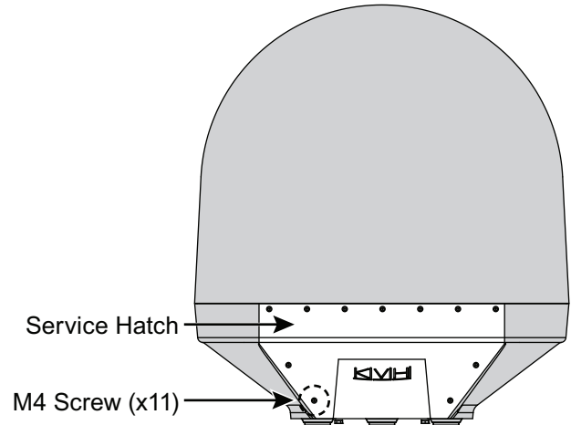
Figure 11: Removing the Radome
