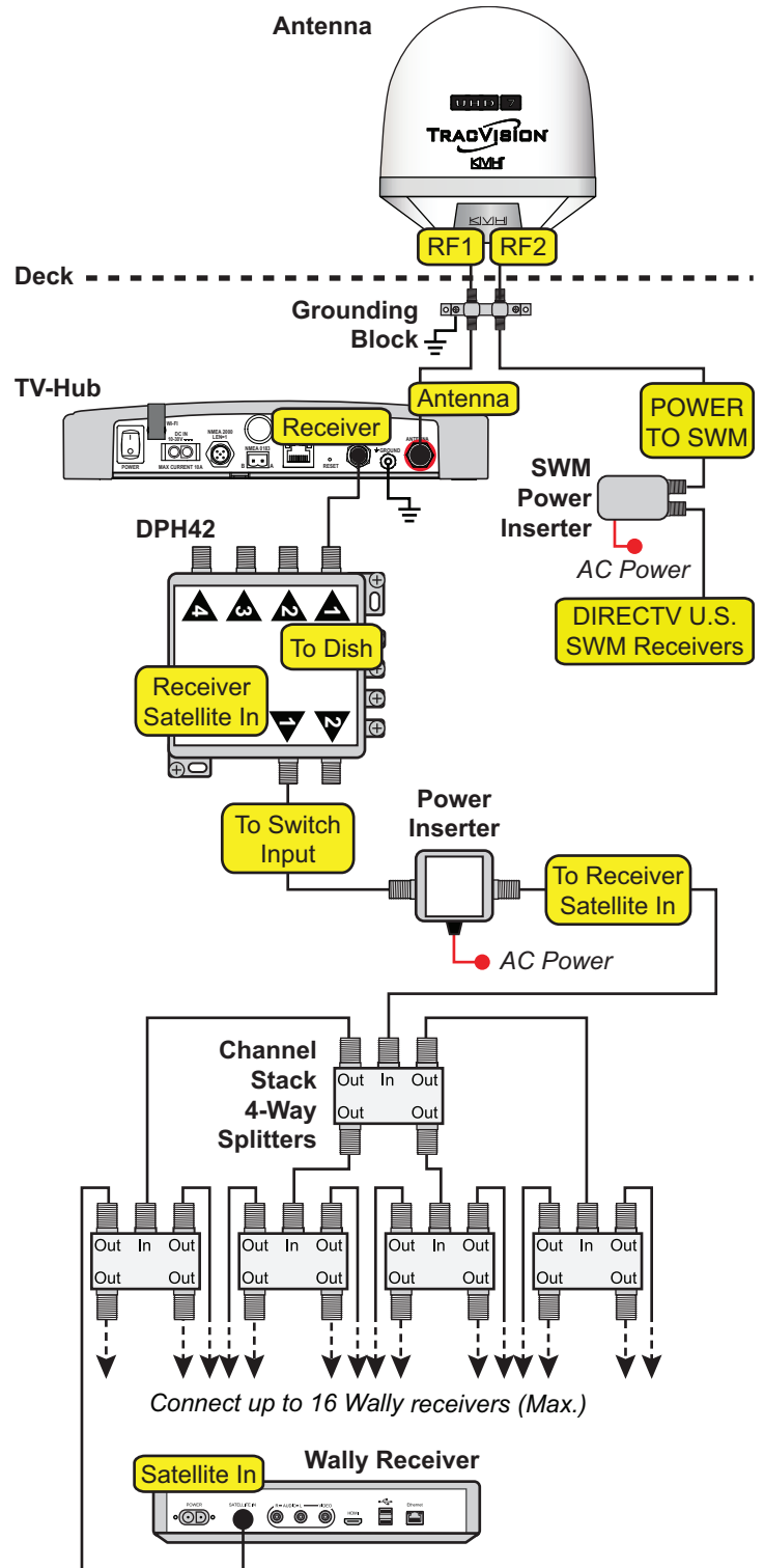
Figure 53: Wiring Up to 16 Wally Receivers
