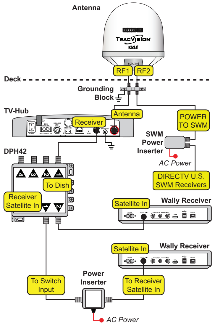
Figure 51: Wiring 1 or 2 DISH Wally Receiver
