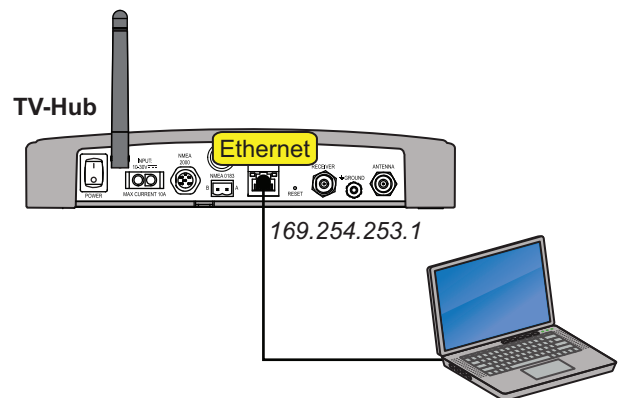
Figure 40: Wired Ethernet Connection
