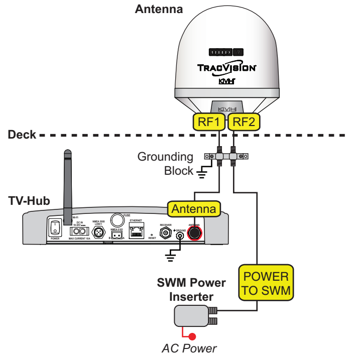
Figure 23: TV-Hub Antenna Connection
