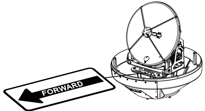
Figure 19: Forward Arrow in Antenna Baseplate
