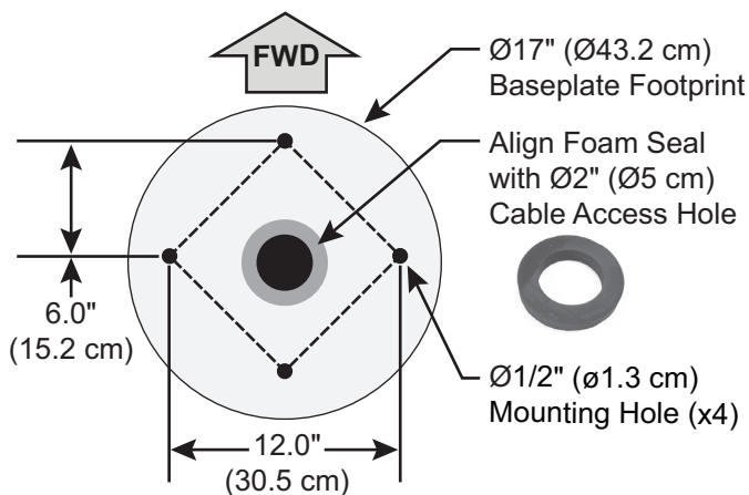
Figure 8: Antenna Mounting Holes Layout
