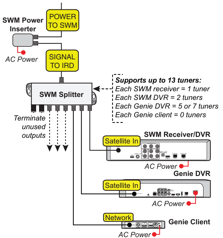
Figure 26: Wiring Up to 8 DIRECTV Receivers
