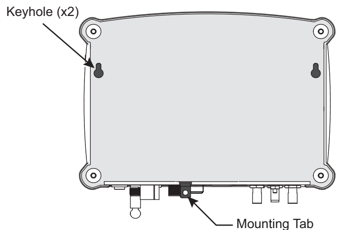
Figure 22: TV-Hub Keyholes and Mounting Tab
