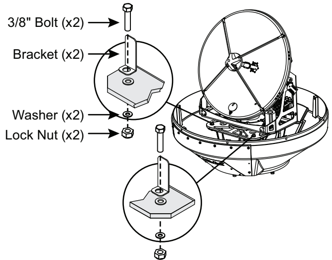
Figure 13: Shipping Restraint Bracket Removal
