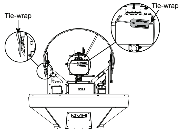
Figure 15: Antenna Restraints
