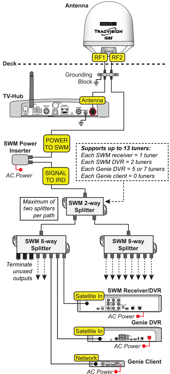
Figure 27: Wiring Up to 13 DIRECTV Receivers
