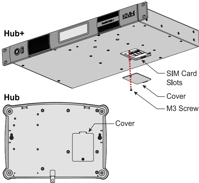
Figure 54: Removing the SIM Card Access Cover
