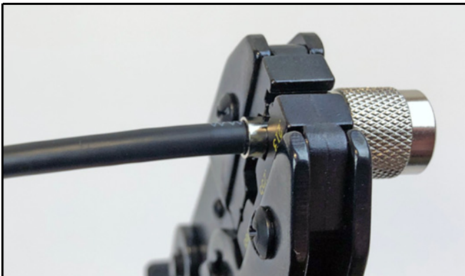
Figure 76: Positioning the Connector in the Crimp Tool
