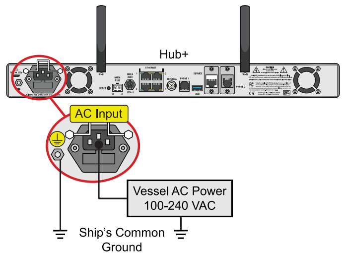
Figure 28: Hub+ AC Power Wiring
