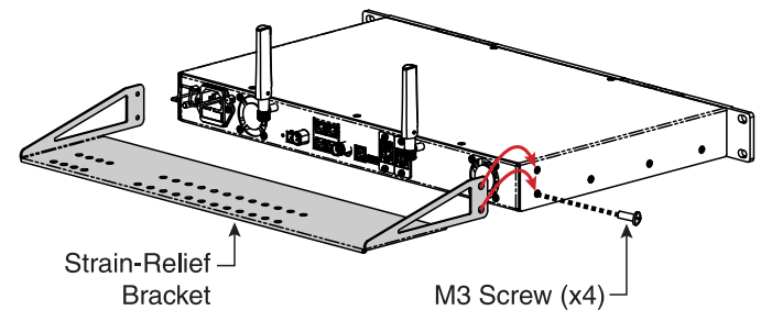
Figure 20: Attaching the Strain-Relief Bracket
