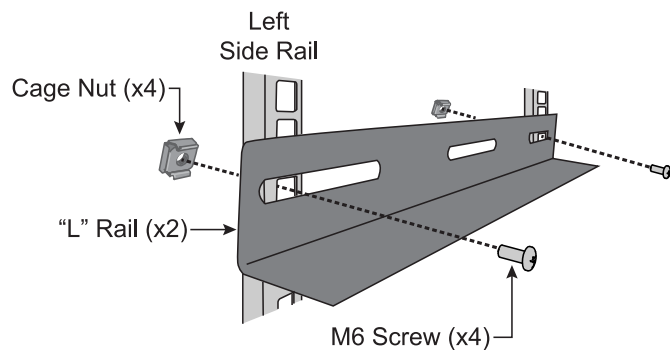
Figure 19: "L" Rail Installation
