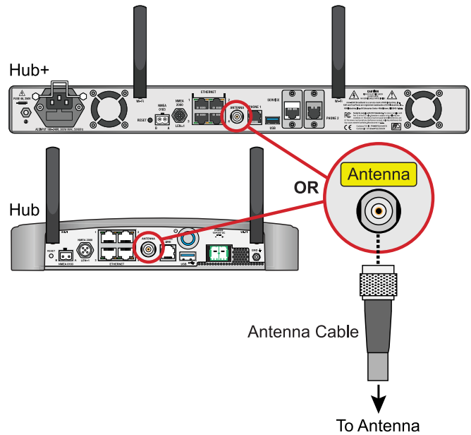
Figure 23: Antenna Cable Connection
