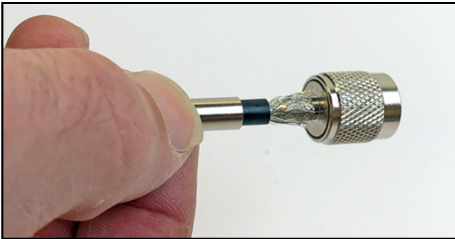
Figure 75: Sliding the Ferrule over the Braid
