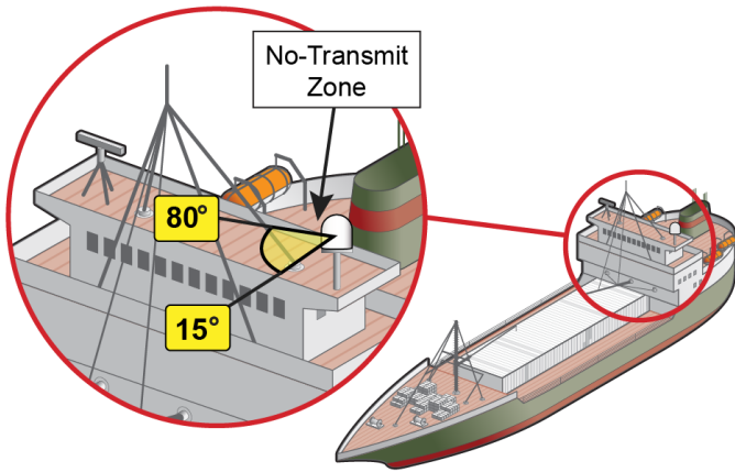
Figure 44: Example of a No-Transmit Zone
