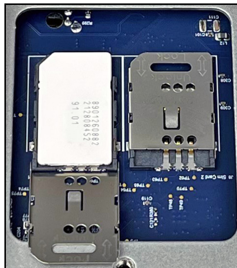
Figure 57: SIM Card Placed in Tray
