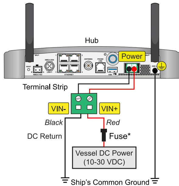
Figure 29: Hub DC Power Wiring
