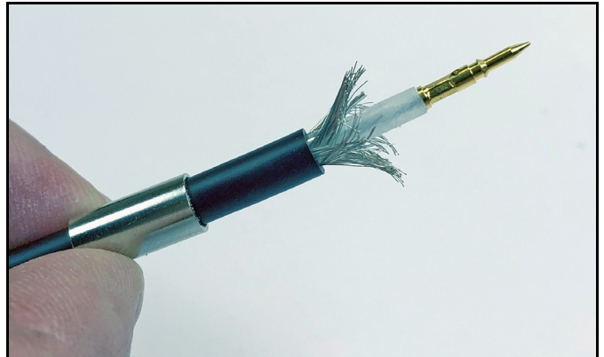
Figure 72: Flared Braid
