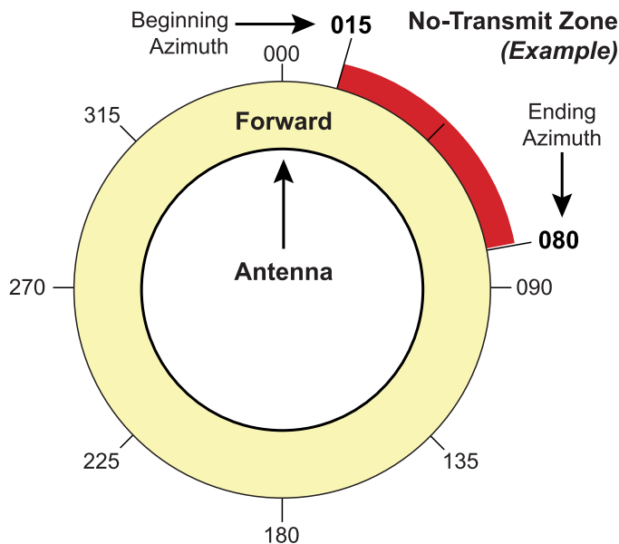
Figure 45: Azimuth Relative to Antenna's Forward Arrow
