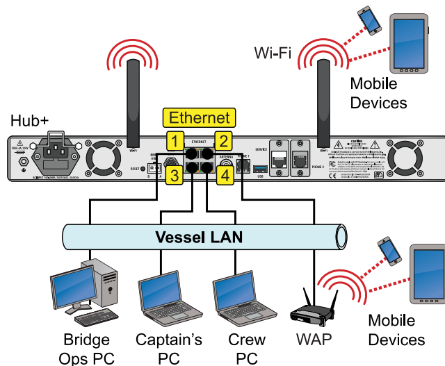
Figure 50: Vessel Network Example (Hub+ Shown)
