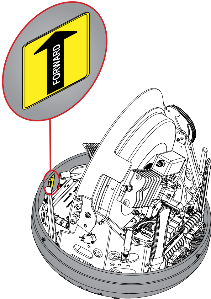
Figure 16: Forward Arrow in Antenna Baseplate
