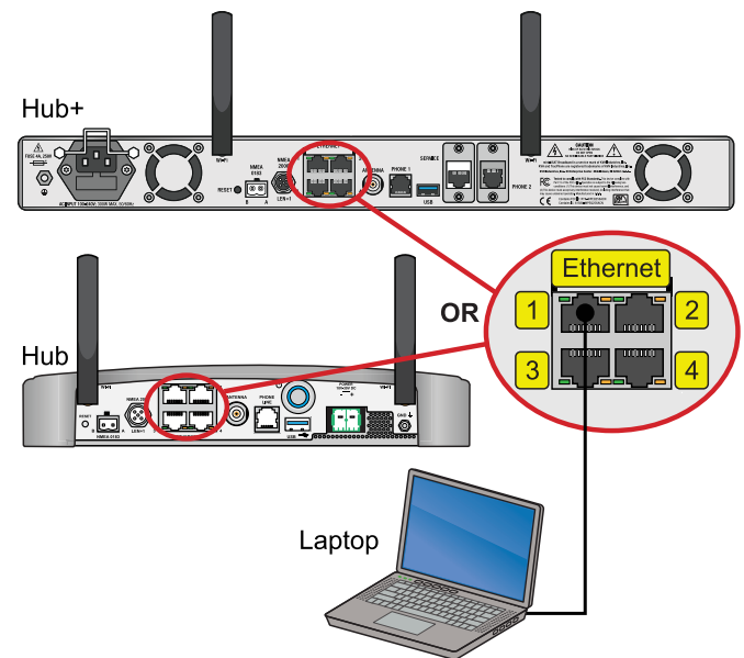
Figure 35: Wired Ethernet Connection
