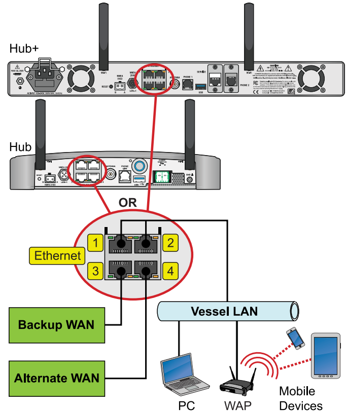
Figure 60: Alternate and/or Backup WAN Connections (Example)
