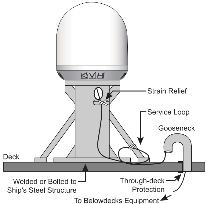
Figure 13: Strain-relief (Finished Installation Example)
