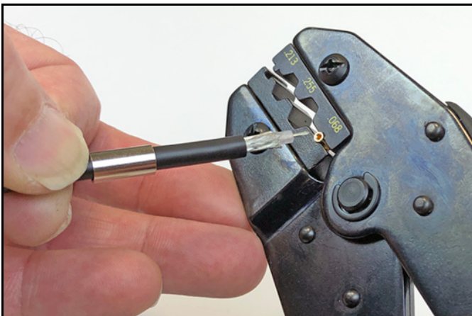
Figure 70: Crimping the Center Pin onto the Center Conductor
