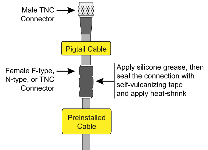
Figure 81: Connecting the Antenna Cable to the Pigtail Cable
