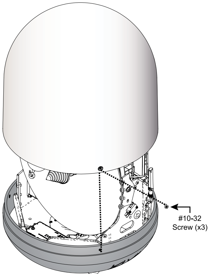
Figure 14: Removing the Radome
