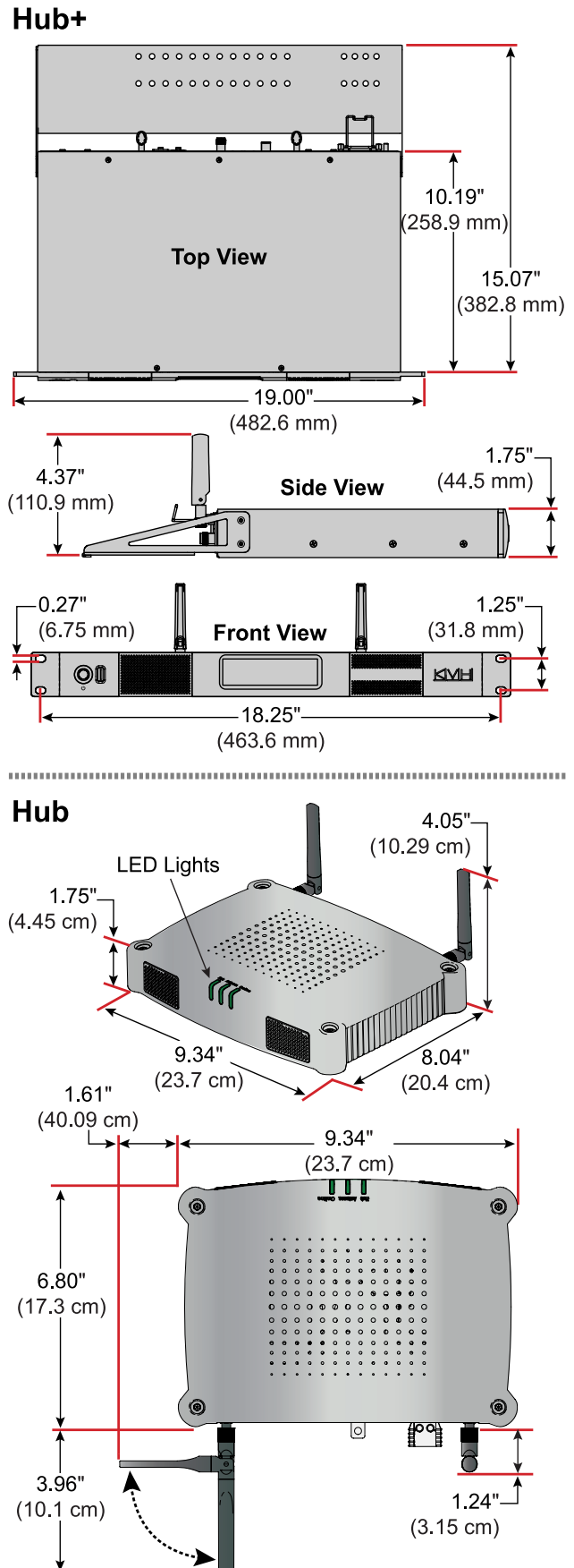
Figure 6: BDU Dimensions
