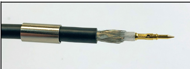
Figure 71: Center Pin Crimped in Place
