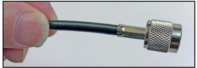
Figure 78: Connector Properly Crimped in Place
