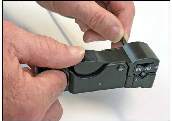
Figure 67: Inserting the Cable into the Stripping Tool
