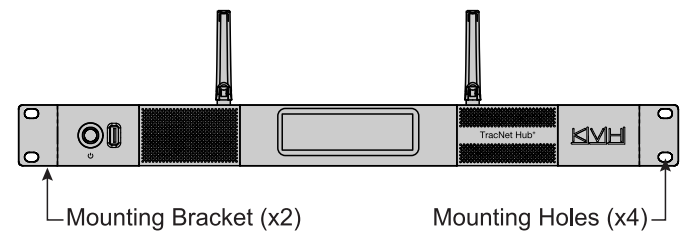
Figure 21: BDU Front Mounting Brackets
