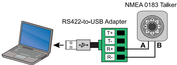
Figure 82: Connecting a NMEA 0183 Talker to a Laptop
