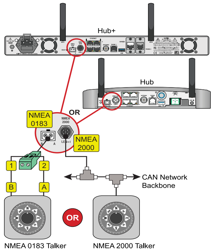
Figure 26: NMEA Wiring
