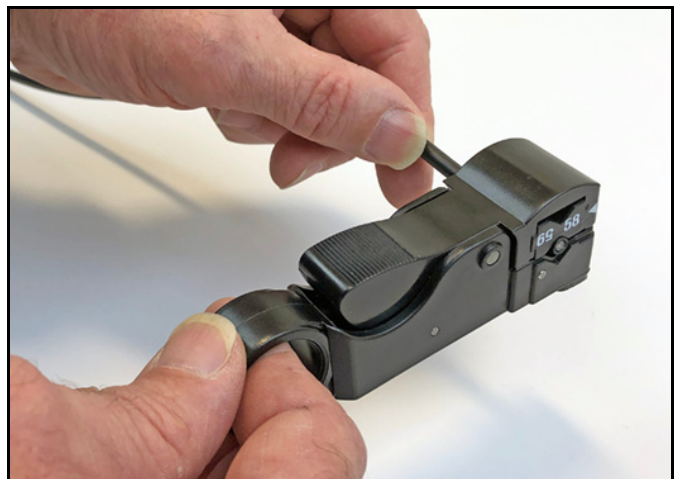
Figure 68: Stripping the Cable
