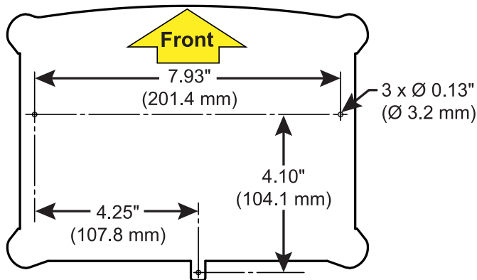
Figure 22: Hub Mounting Template
