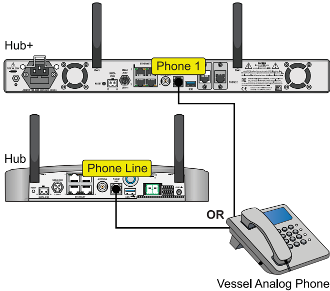
Figure 51: Connecting the Vessel Phone (Example)
