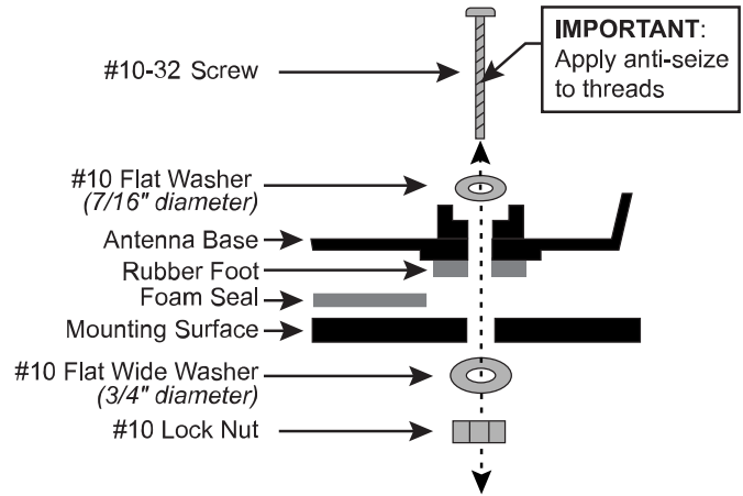
Figure 11: Mounting Hardware
