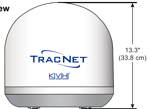
Figure 2: Antenna Dimensions
