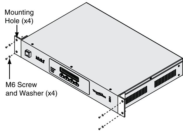
Figure 19 ACU Equipment Rack Mounting
