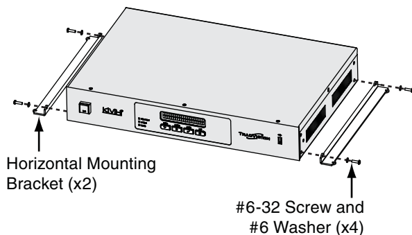
Figure 21 ACU Horizontal Surface Mounting
