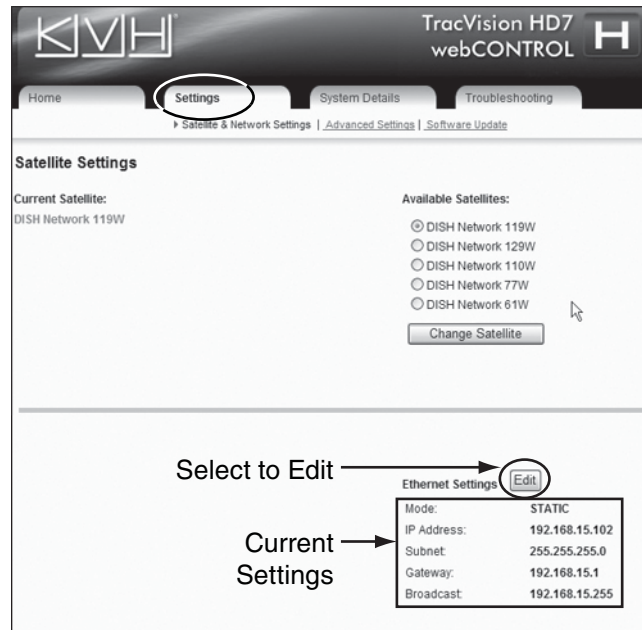
Figure 33 Ethernet Settings on the Web Interface
