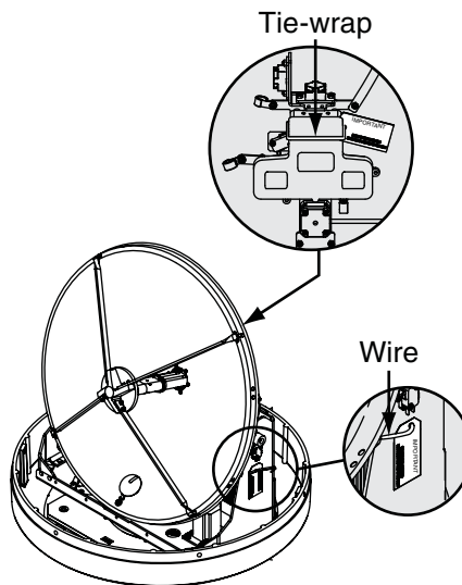
Figure 18 Shipping Restraints
