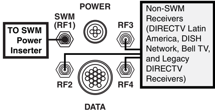
Figure 13 Antenna Connectors
