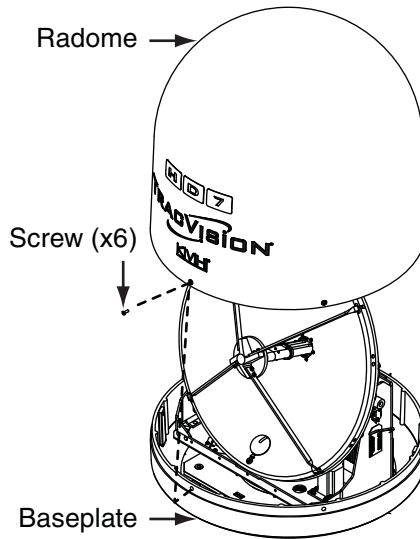
Figure 10 Radome Screws
