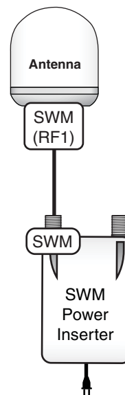
Figure 23 Antenna SWM (RF1) Wiring
