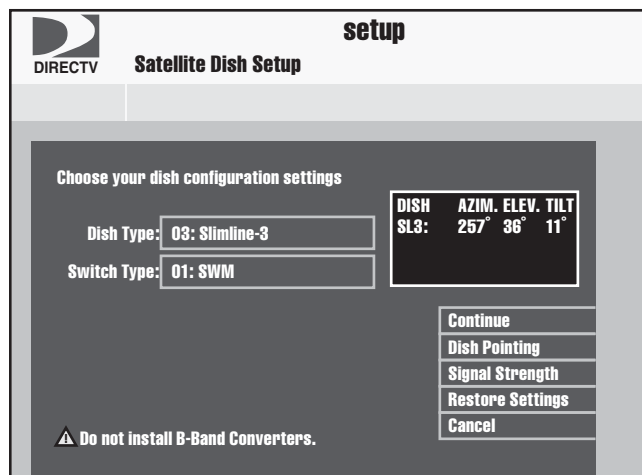
Figure 28 DIRECTV SWM Receiver/DVR Configuration
