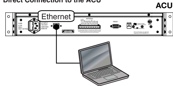
Figure 30 Connection Options
