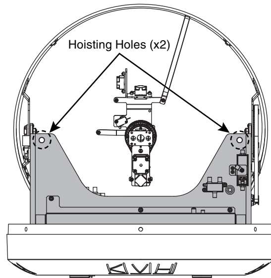
Figure 12 Antenna Hoisting Holes
