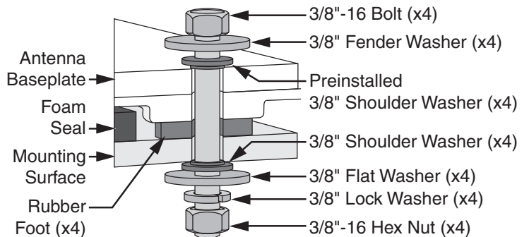
Figure 17 Antenna Mounting
