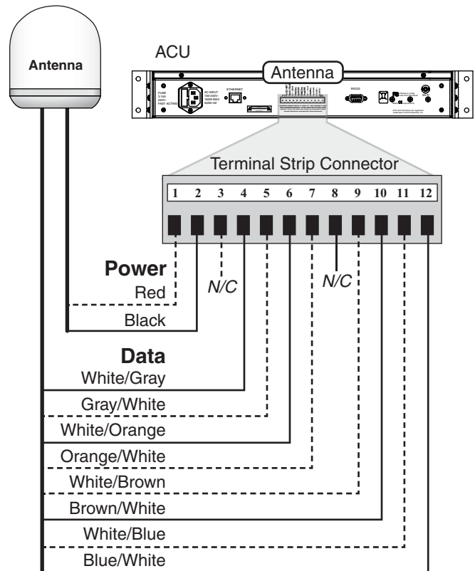
Figure 22 Antenna Power and Data Wiring
