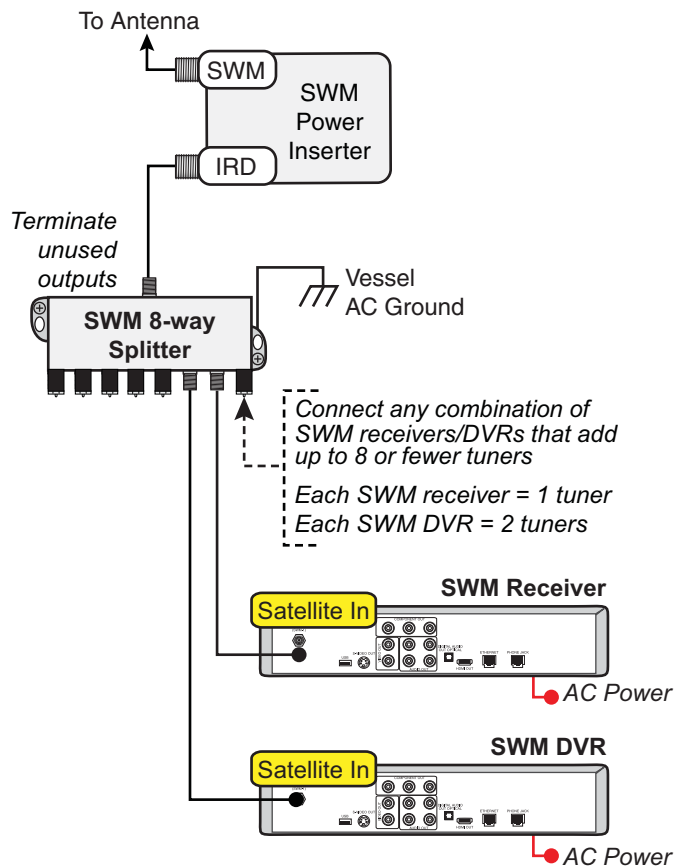
Figure 26 DIRECTV SWM Receiver/DVR Wiring (Example)
