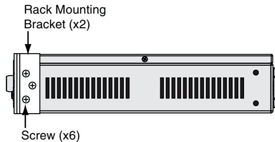
Figure 20 ACU Rack Mounting Bracket Removal
