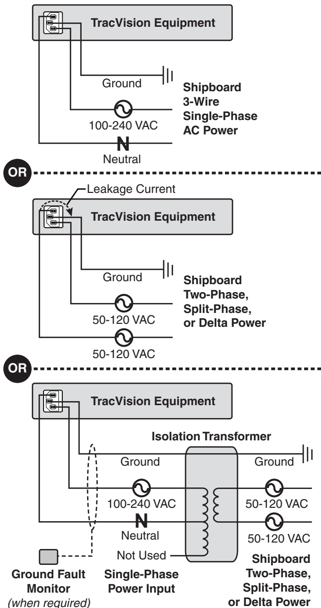
Figure 24 AC Power Options
