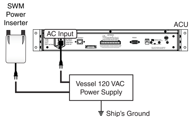
Figure 25 Power Wiring
