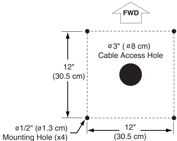
Figure 6 Antenna Mounting Holes Layout
