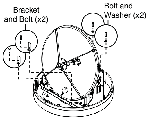
Figure 11 Shipping Restraints
